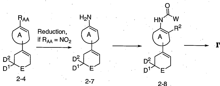
Scheme 2b
