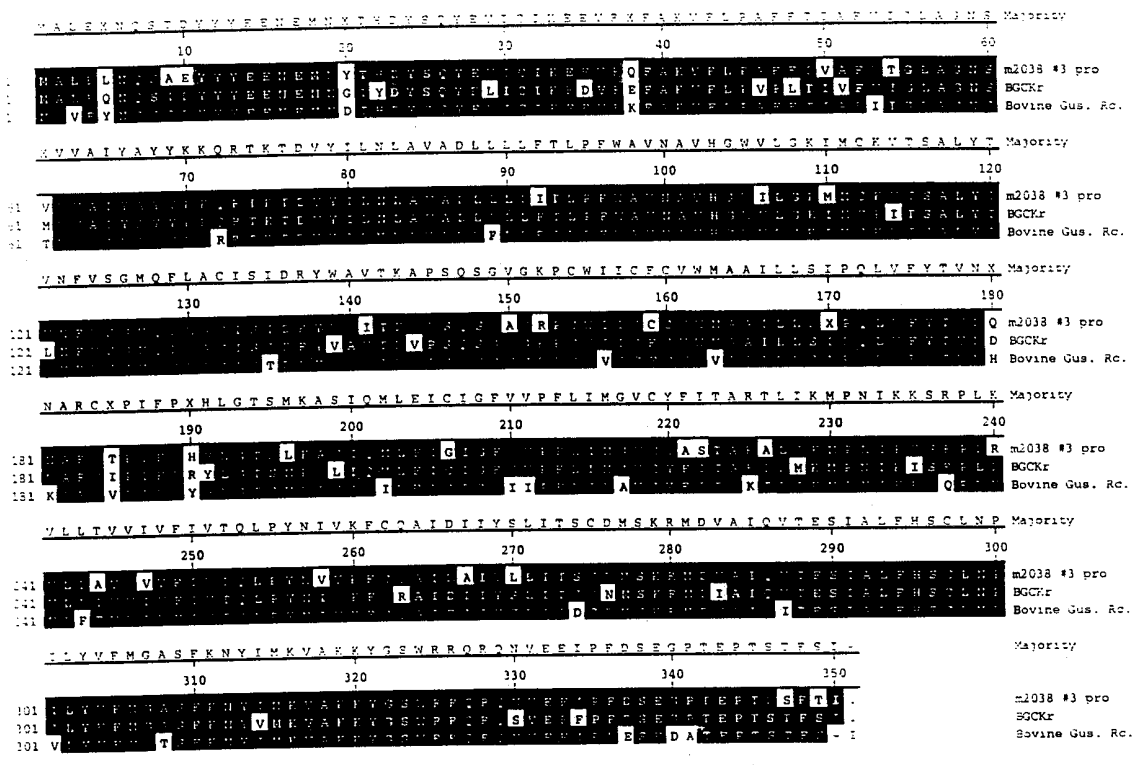
Decoration 'Decoration #1': Shade (with solid black) residues that match the Consensus exactly.
