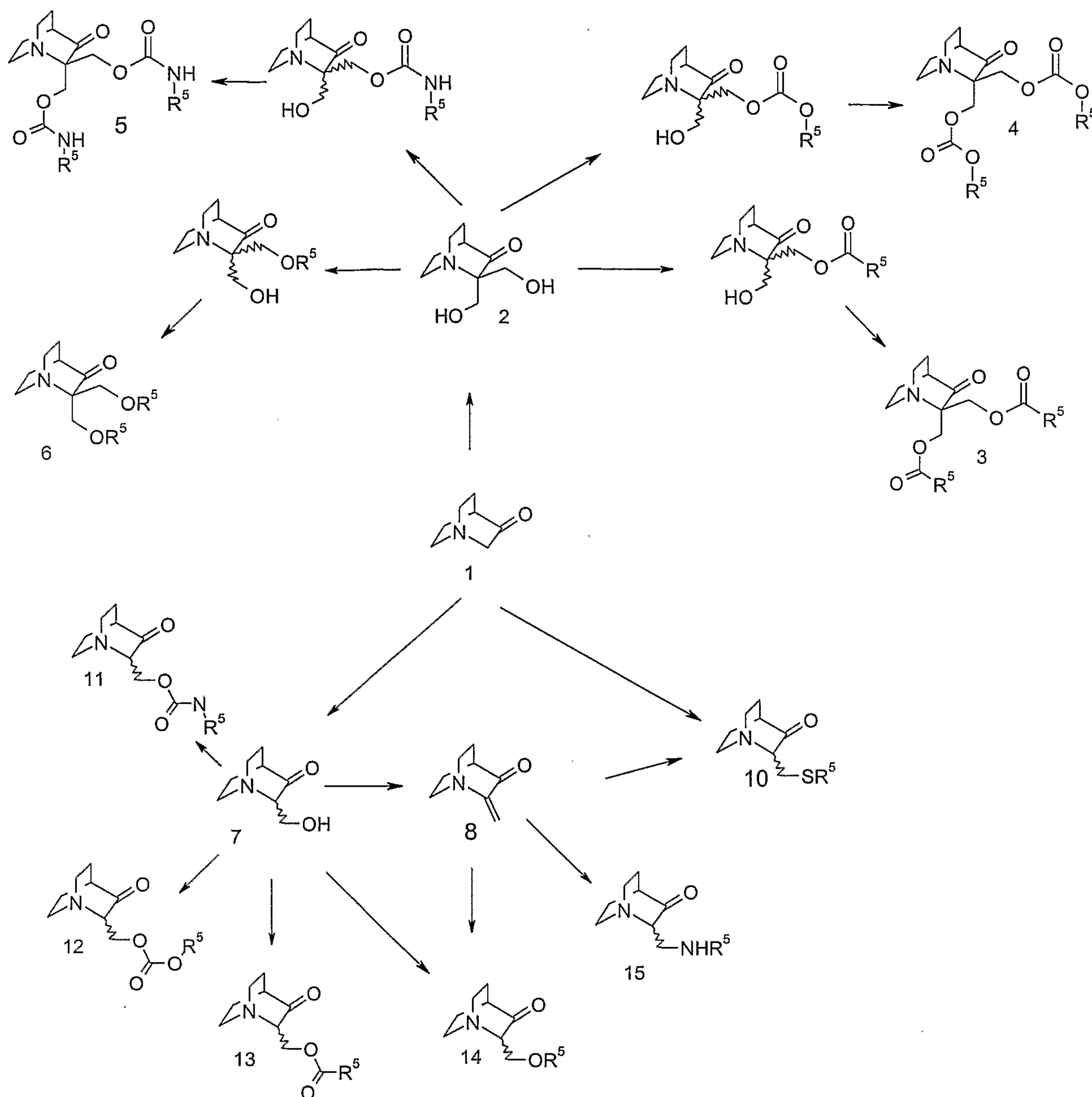
Reaction Scheme 2
