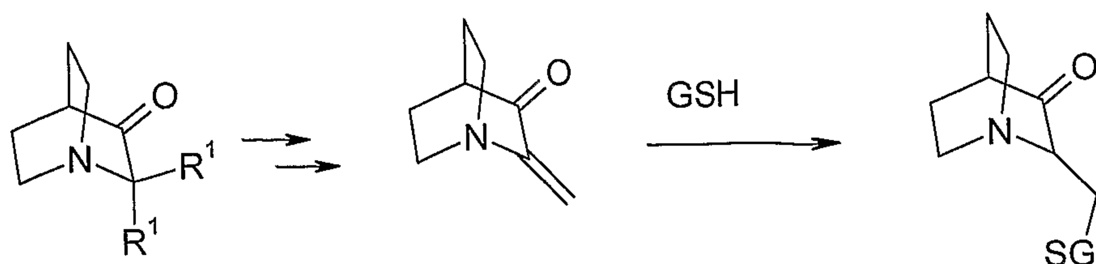
Reaction Scheme 1
