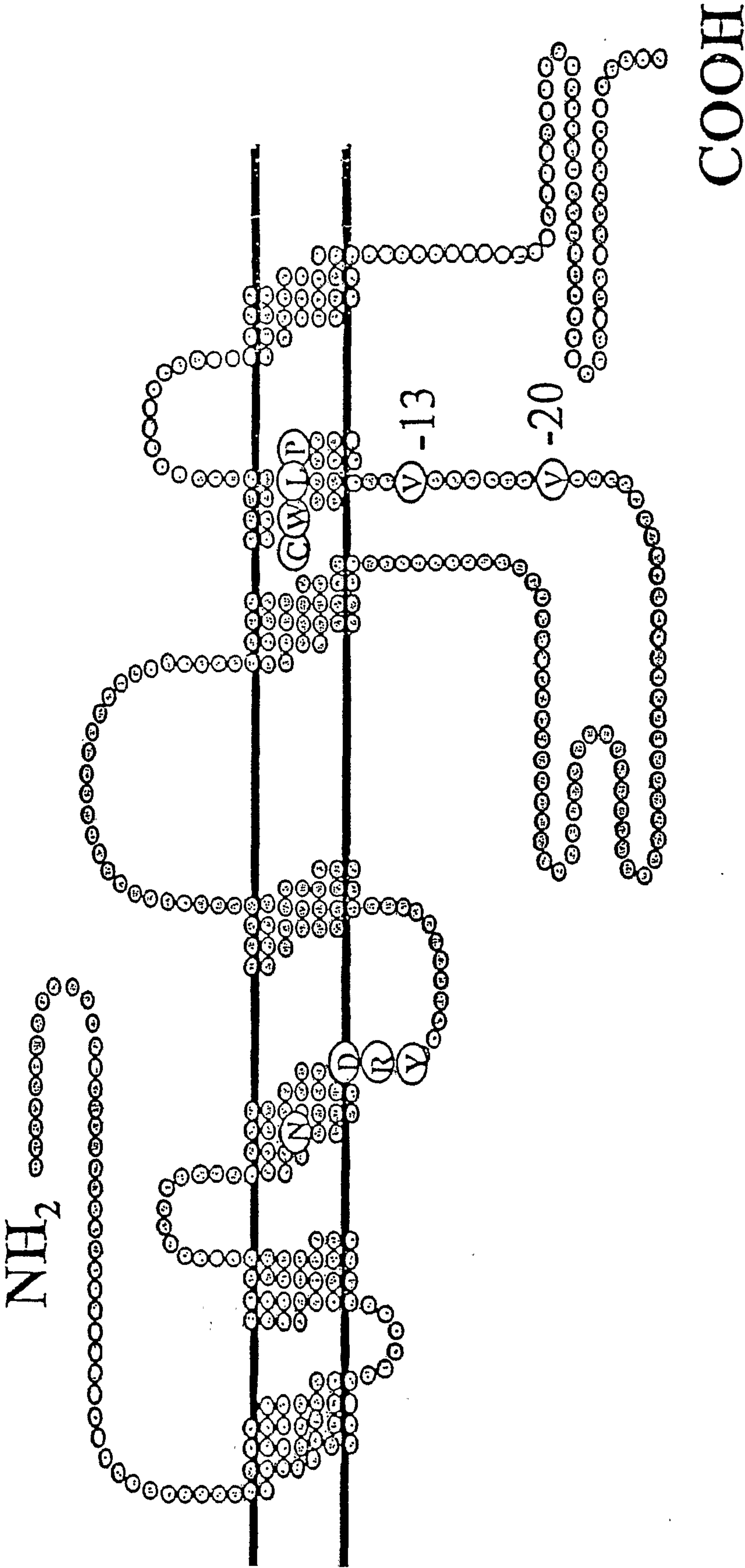
Target Residues Within Class I GPCRs
