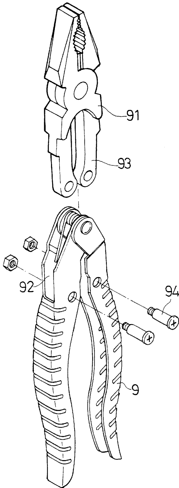
FIG. 6 PRIOR ART
