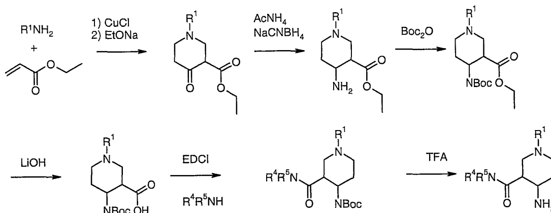
Scheme 7
