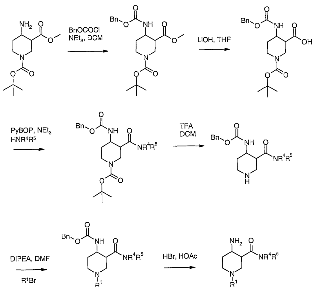
Scheme 5
