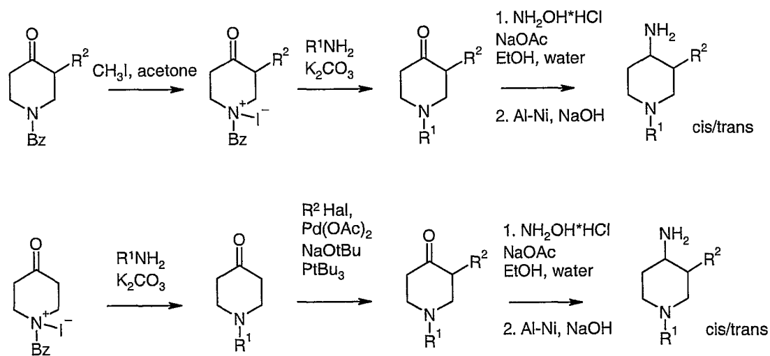
15 Scheme 4
