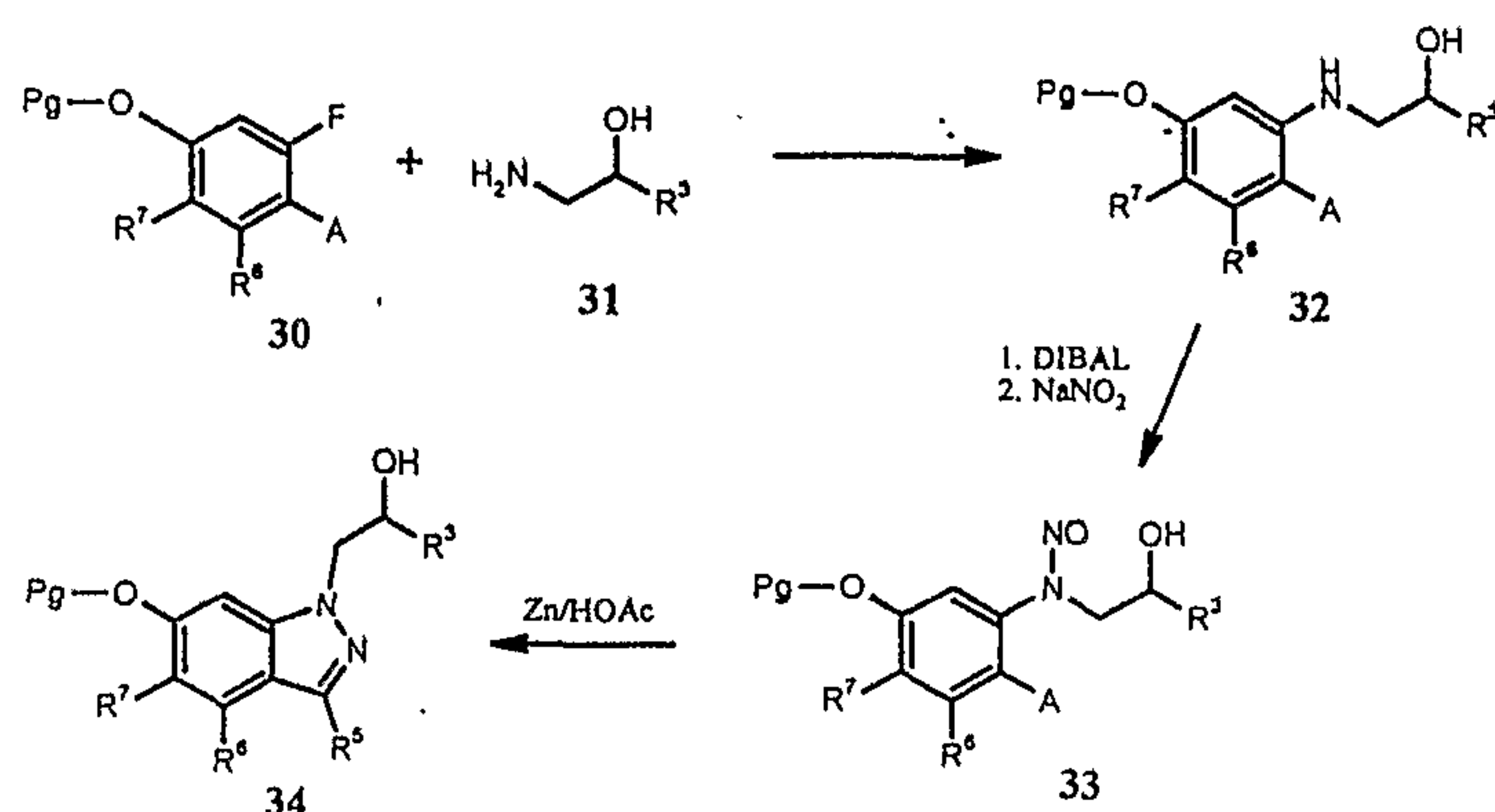
Scheme 6
