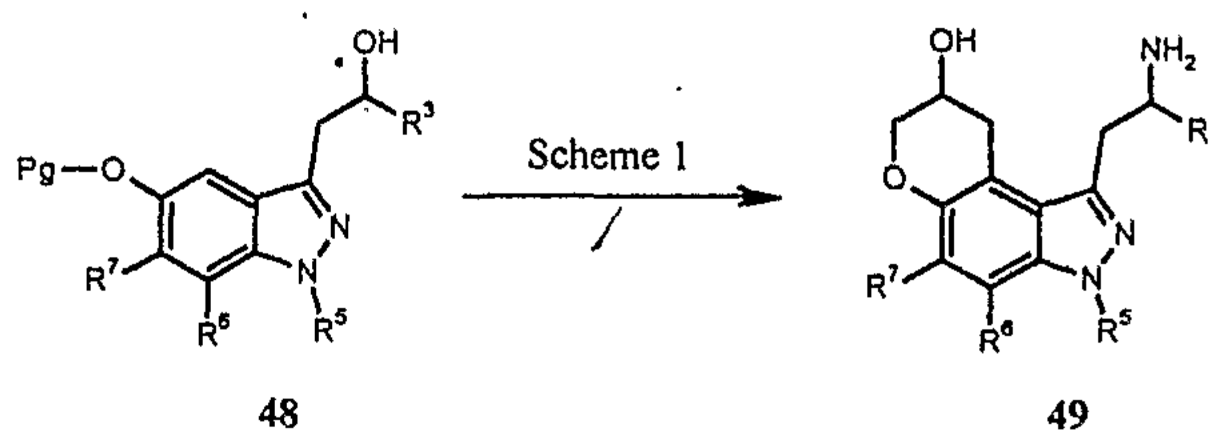
Scheme 11
