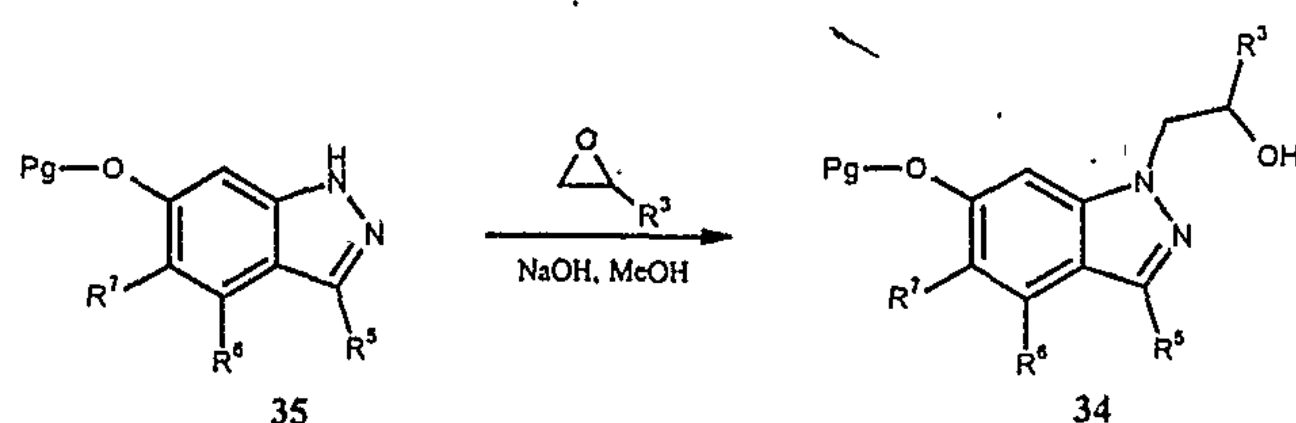
Scheme 7
