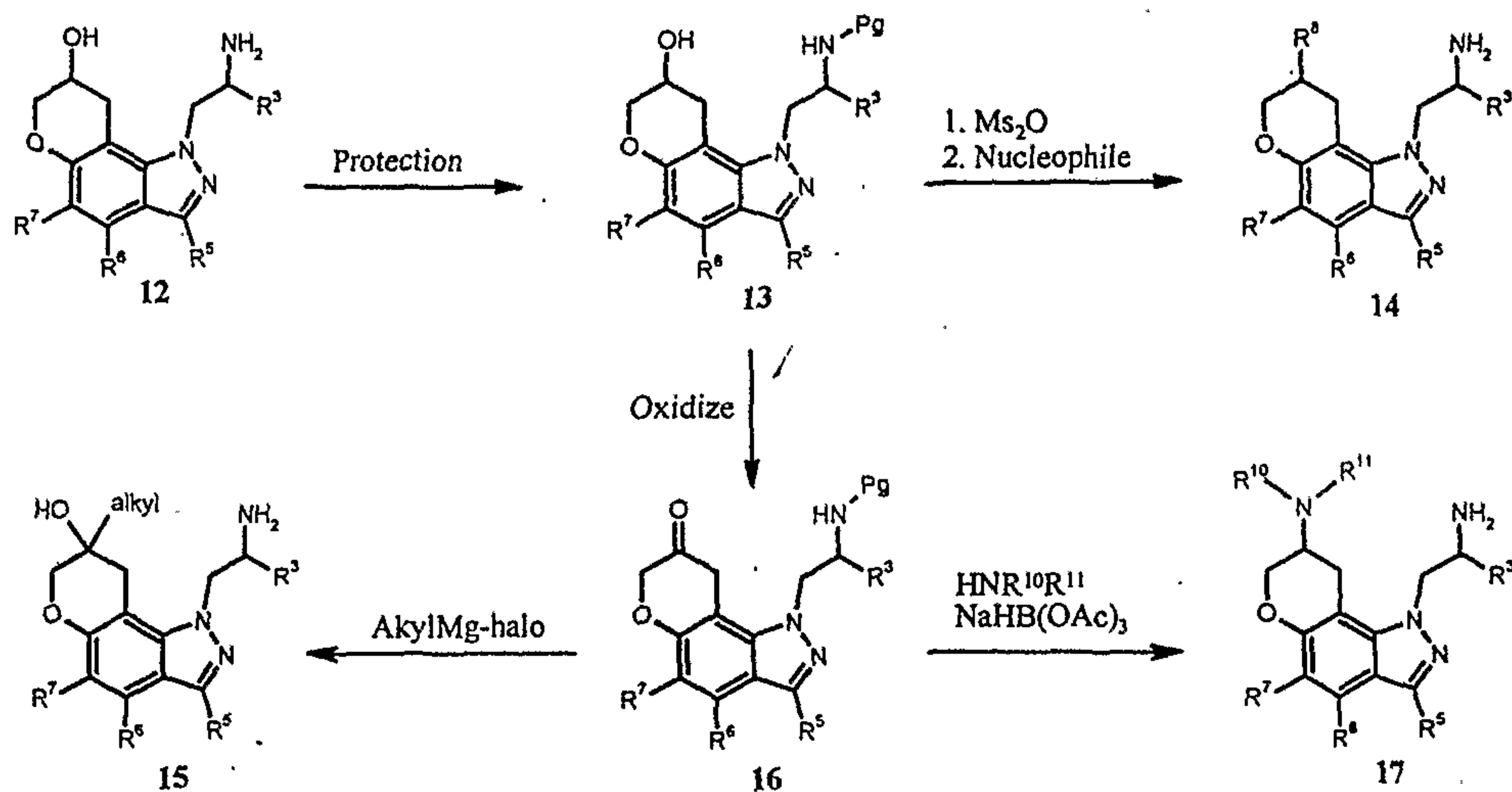
Scheme 2
