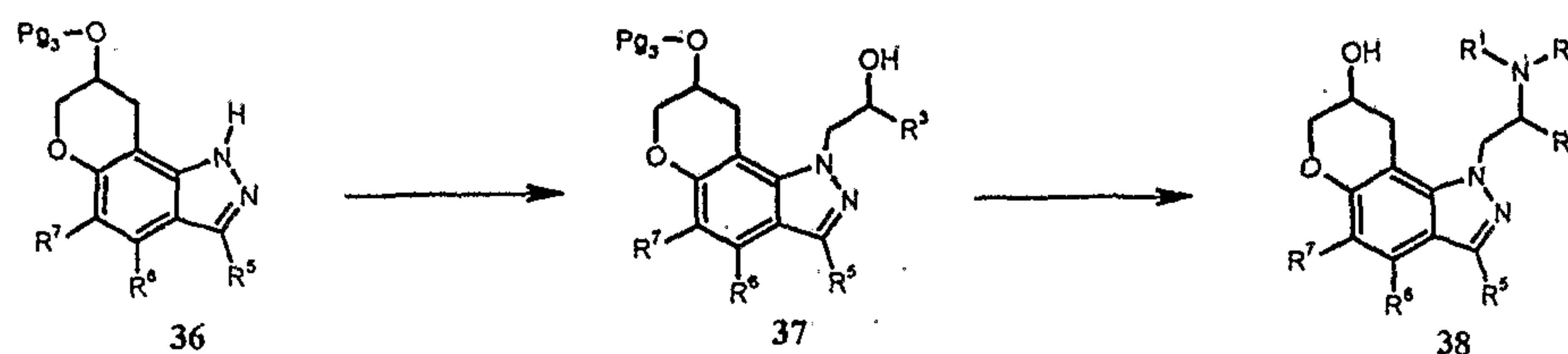
Scheme 8
