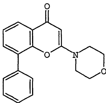
LY294002
