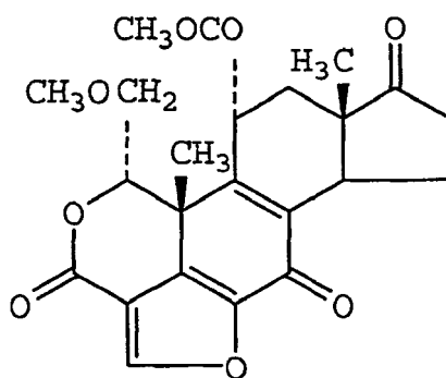
wortmannin
