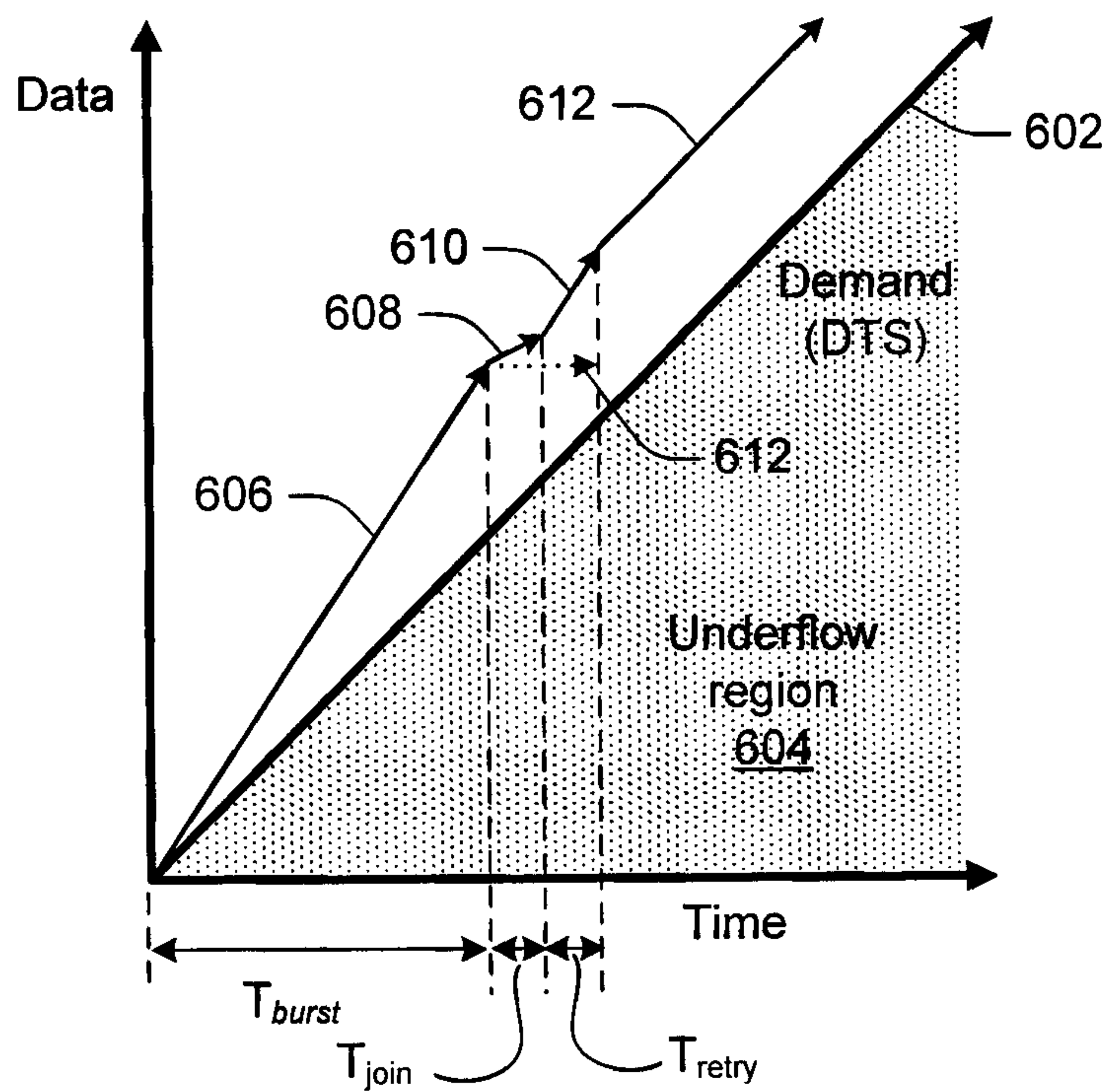
SCENARIO 1-B: Sample data consumption graph for rate-limited ACC ( E=.25 , T_{burst} = 6 , T_{join} = 1 )
