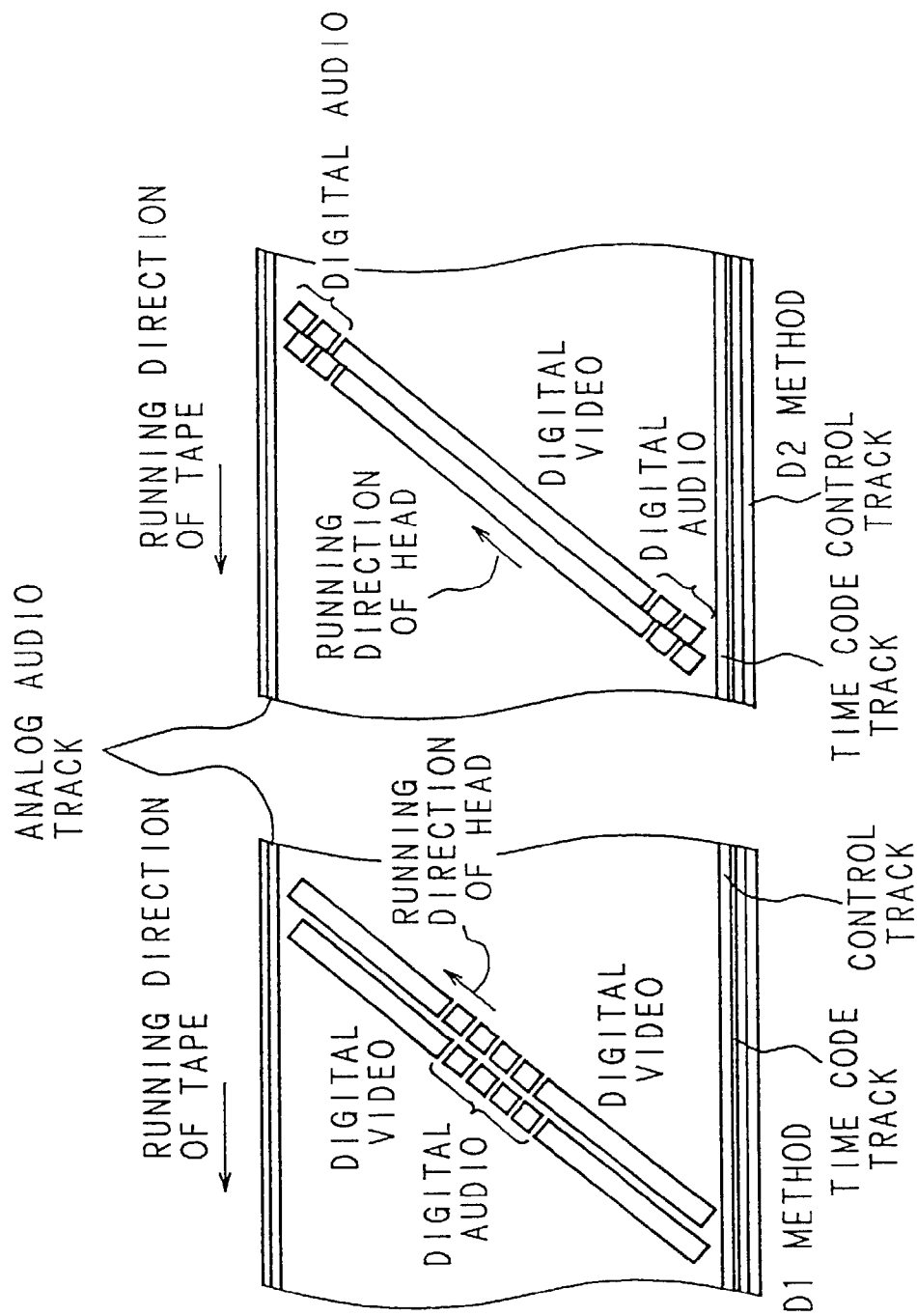
Fig. 18 Prior Art
