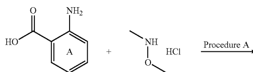
Scheme II: Synthesis of N-(2-Benzoyl-Phenyl)-Benzenesulfonamides and N-(2-Benzoyl-Phenyl)-Heteroarylsulfonamides.
