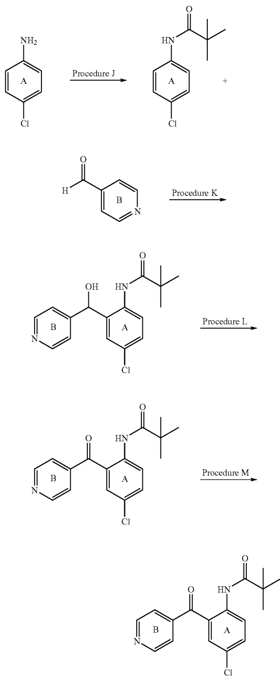
Scheme V: Synthesis of (2-amino-5-chloro-phenyl)-pyridin-4-yl-methanones
