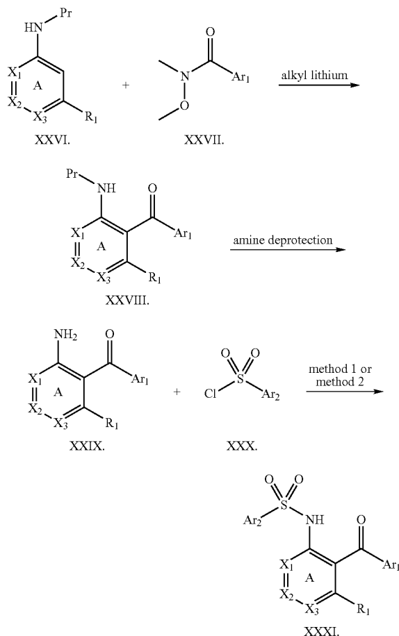
Scheme I: General synthesis of diaryl methanones.
