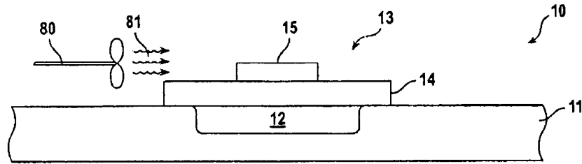
FIG. 1 (PRIOR ART)
