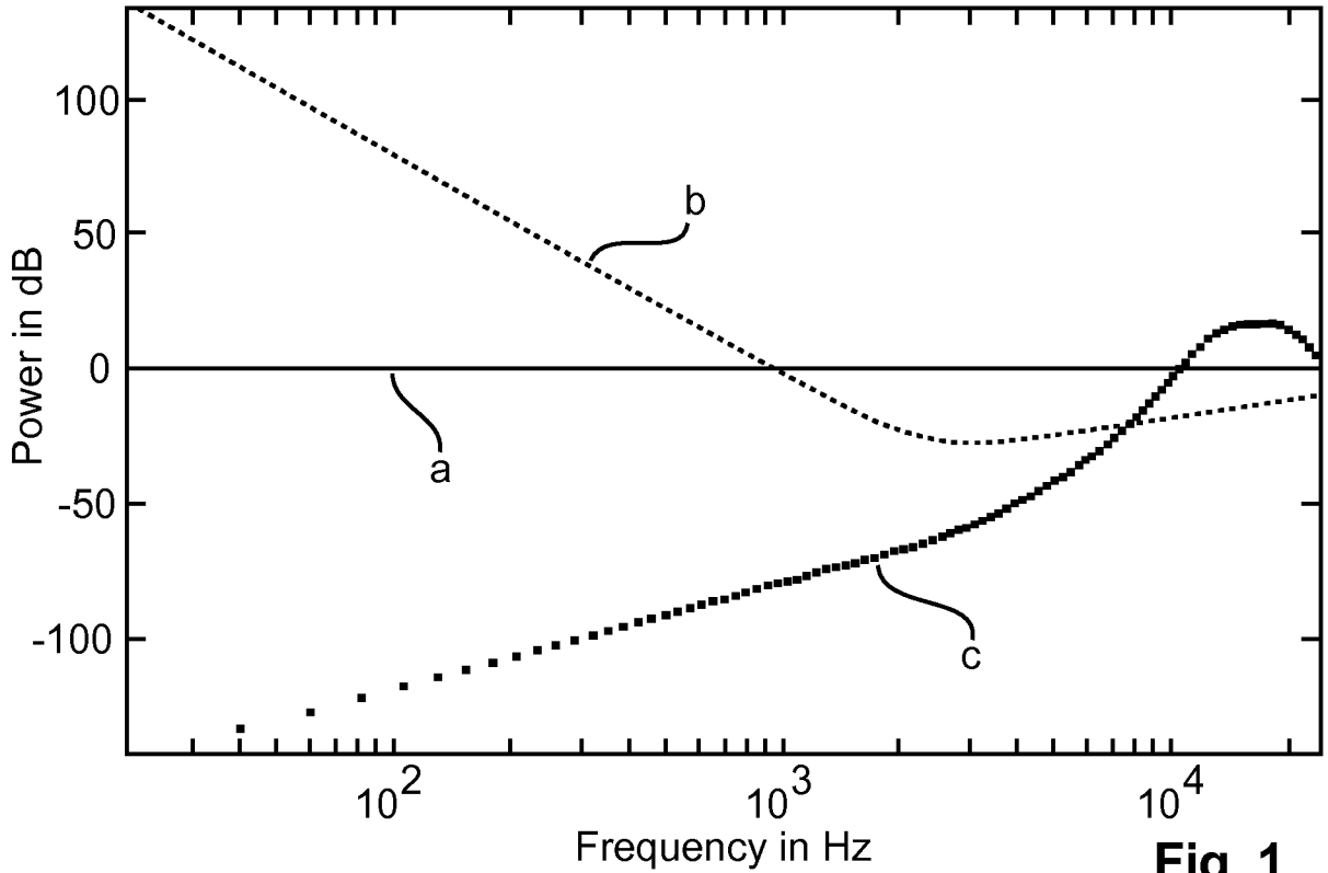
Components of the Resulting Loudspeaker Weight (SNR=20dB)
