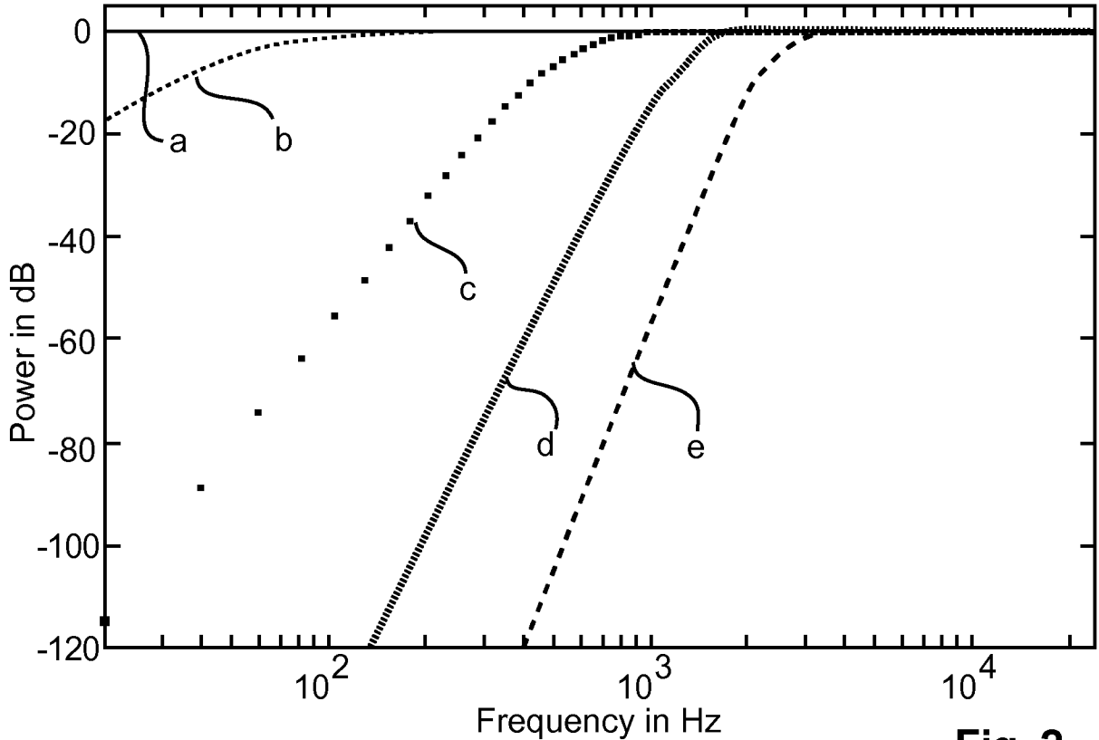
Noise Reduction Filters (SNR=20 dB)
