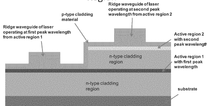
An example of a layered active region configuration where adjacent lasers are operating at different wavelengths as a result of lasing off of two different active regions with different peak wavelengths
