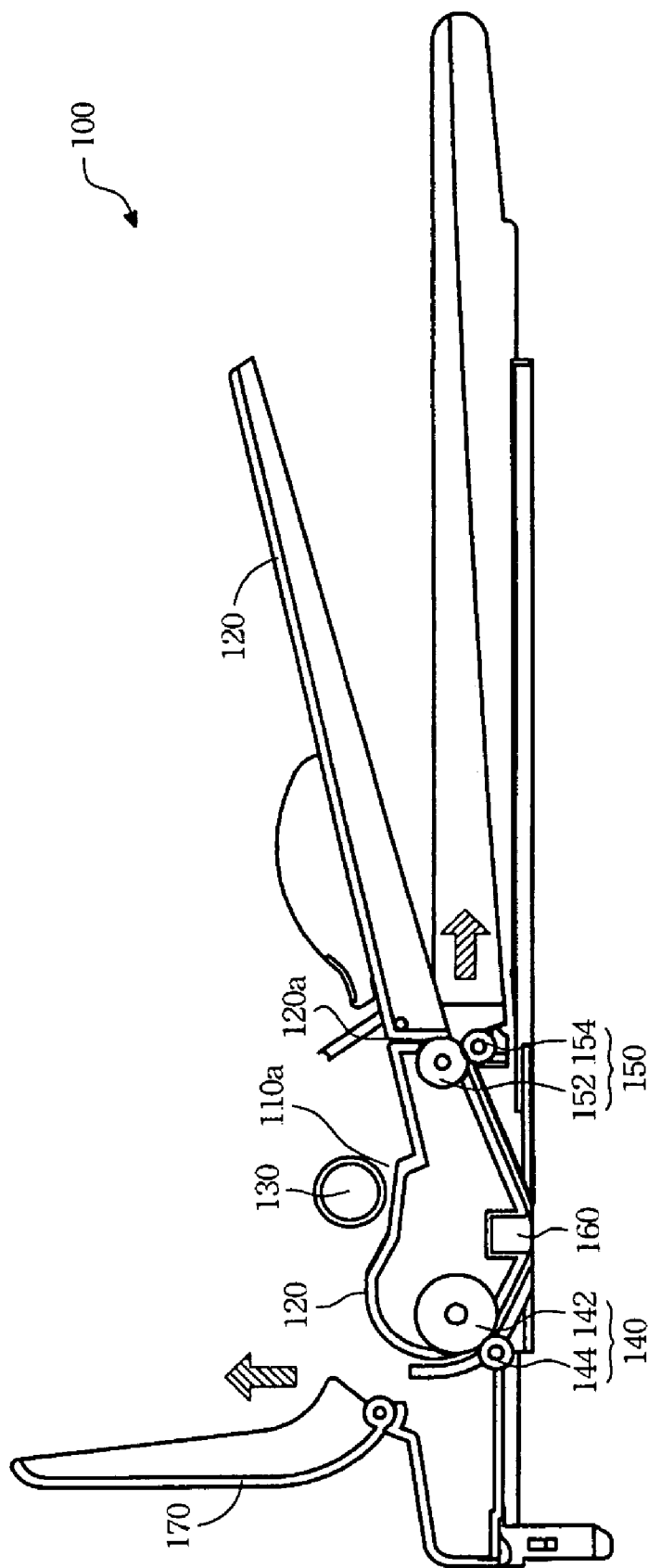
FIG. 2 (Prior Art)
