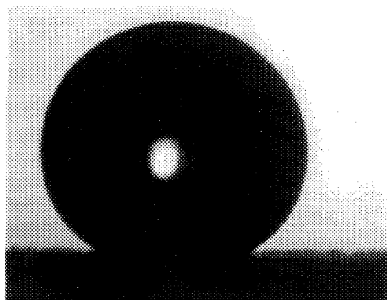
CONTACT ANGLE OF WATER WITH APD - FLUOROPOLYMER (145°)
