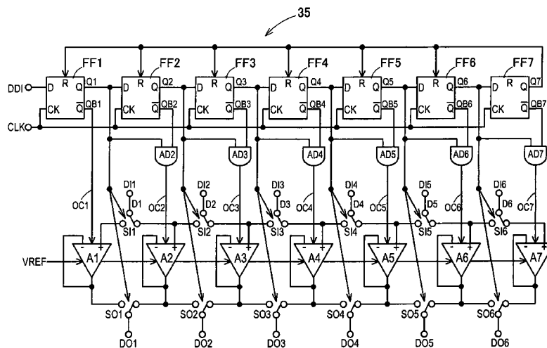
SCHEMATIC DIAGRAM OF CIRCUIT BLOCK DIRECTED TO SECOND EMBODIMENT
