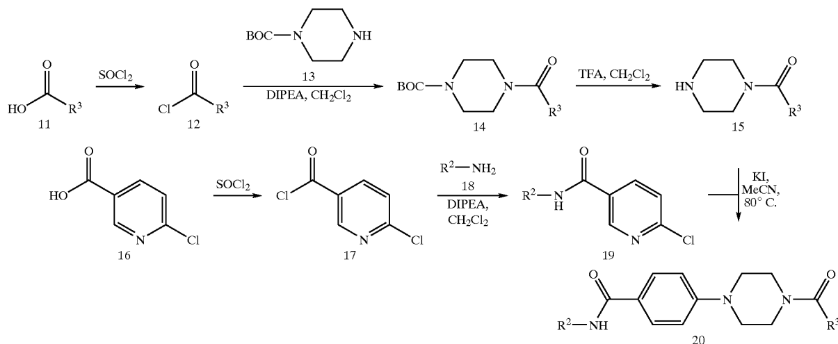
REACTION SCHEME 2
