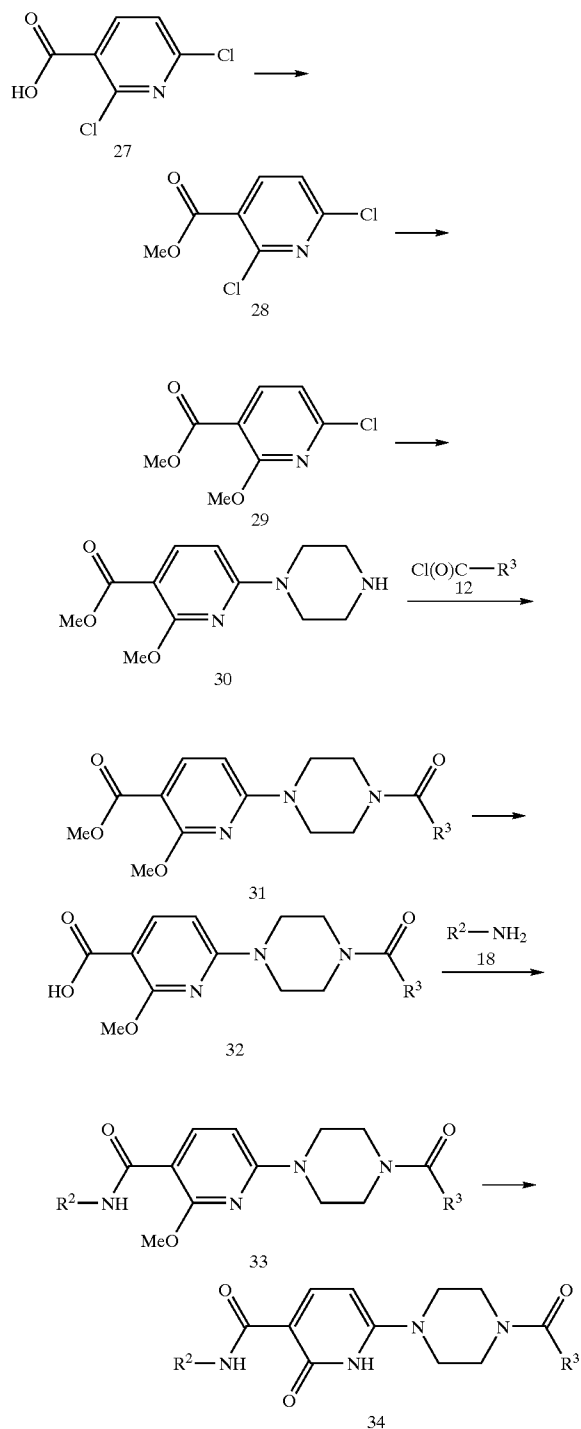
REACTION SCHEME 4
