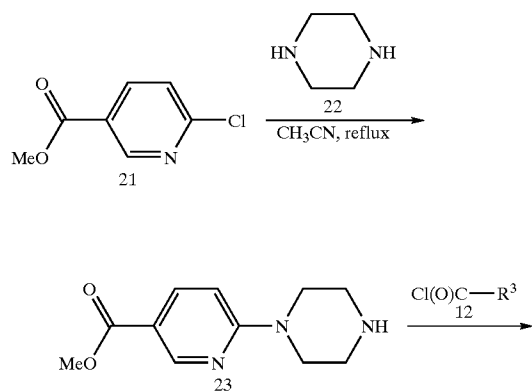
REACTION SCHEME 3
