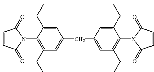
di(3,5-diethyl-4-maleimidophenyl)methane
