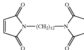
dodecane N,N'-bismaleimide
