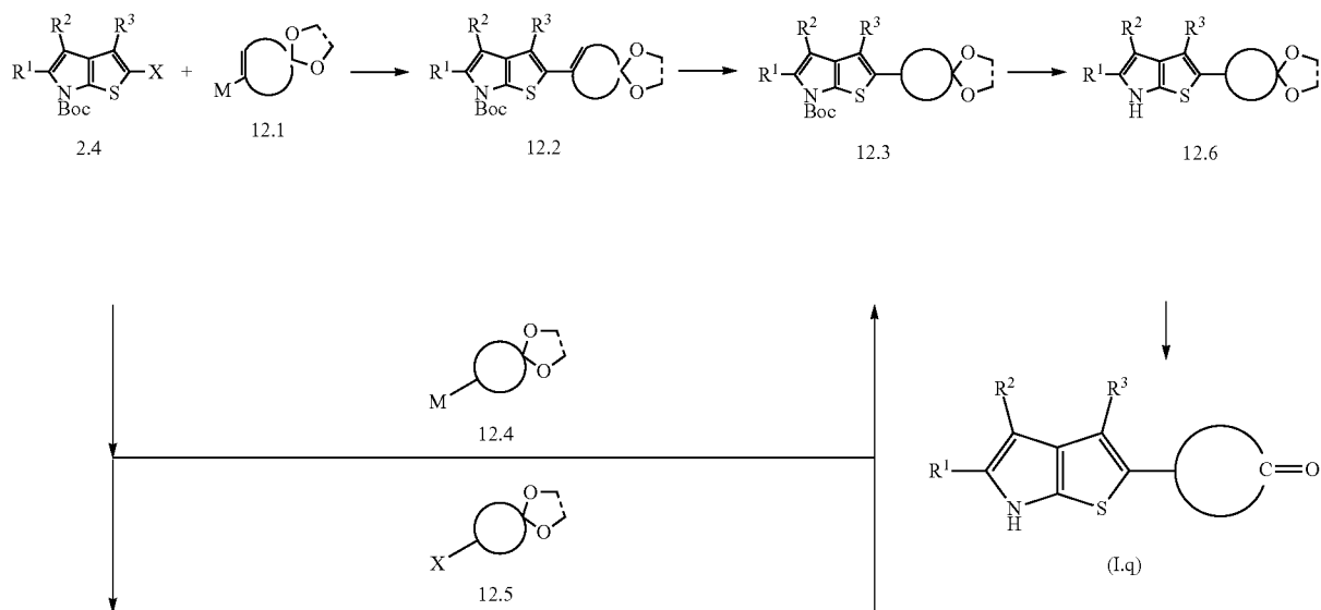
General Reaction Scheme 12
