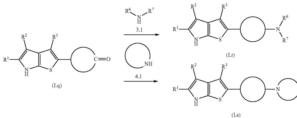
General Reaction Scheme 13
