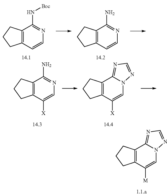
General Reaction Scheme 14
