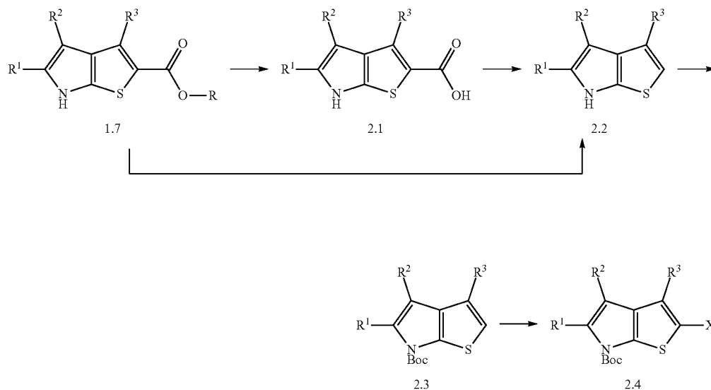
General Reaction Scheme 2
