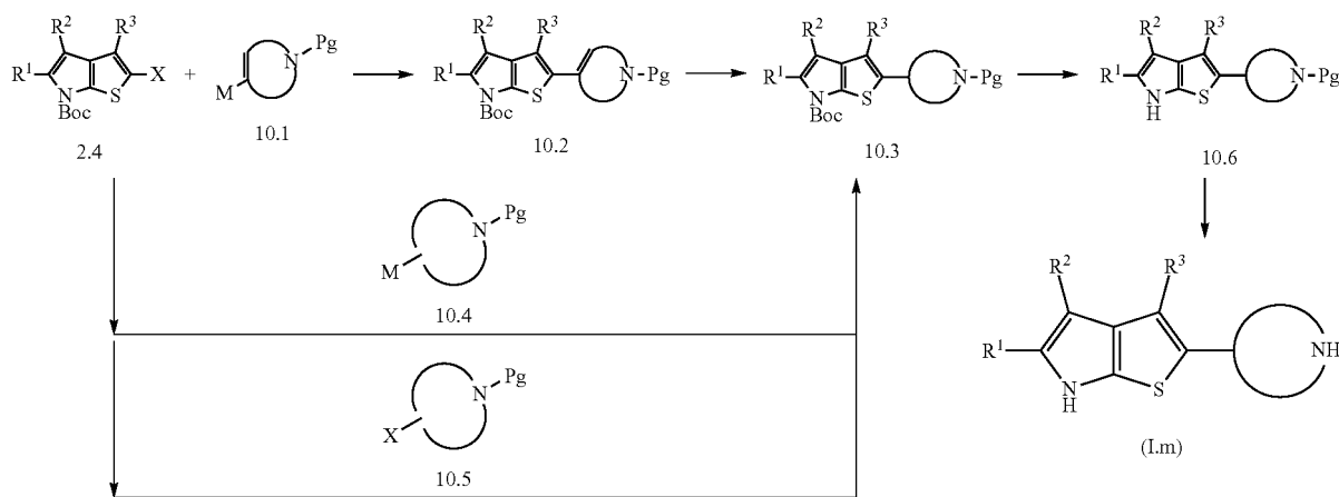
General Reaction Scheme 10
