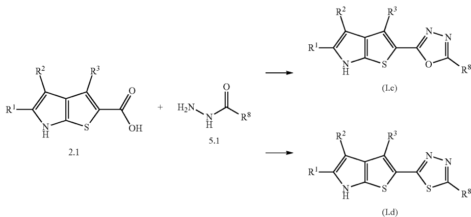
General Reaction Scheme 5
