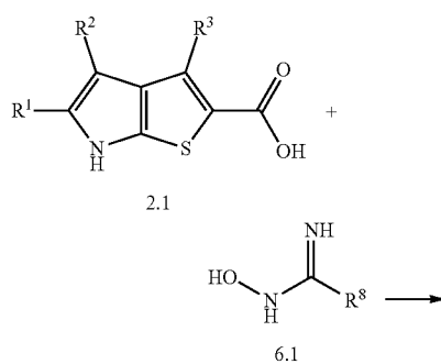
General Reaction Scheme 6
