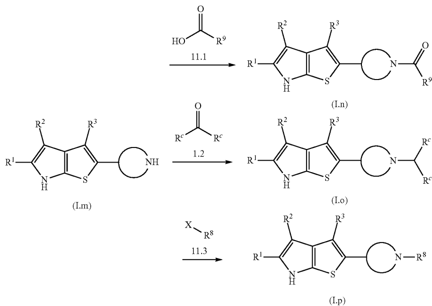
General Reaction Scheme 11
