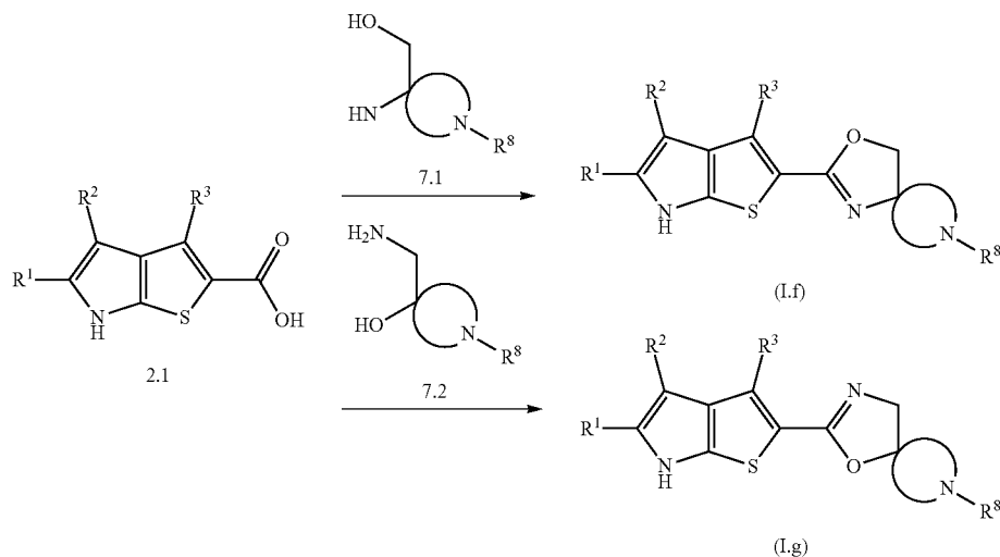
General Reaction Scheme 7
