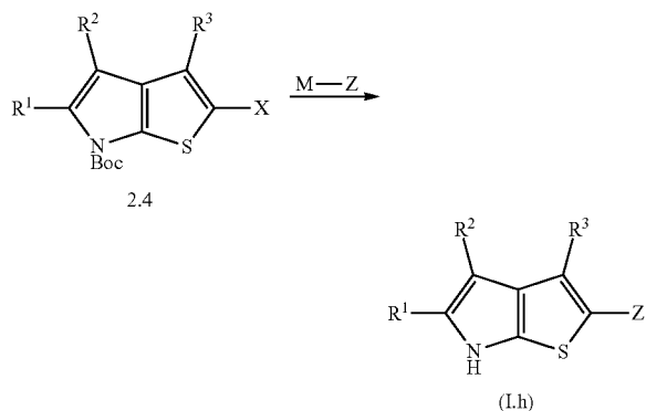
General Reaction Scheme 8
