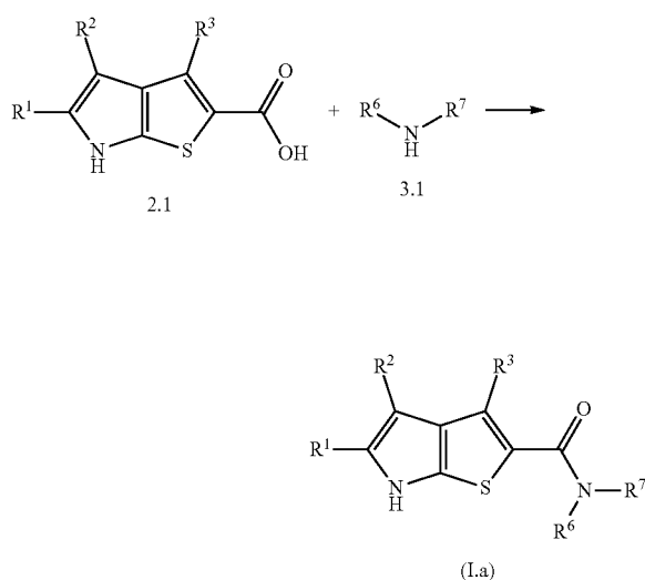
General Reaction Scheme 3
