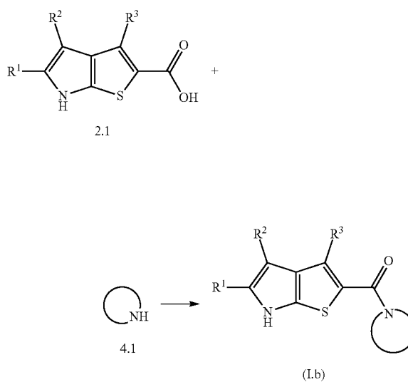
General Reaction Scheme 4
