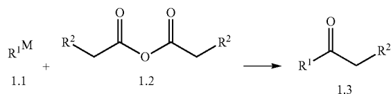
General Reaction Scheme 1
