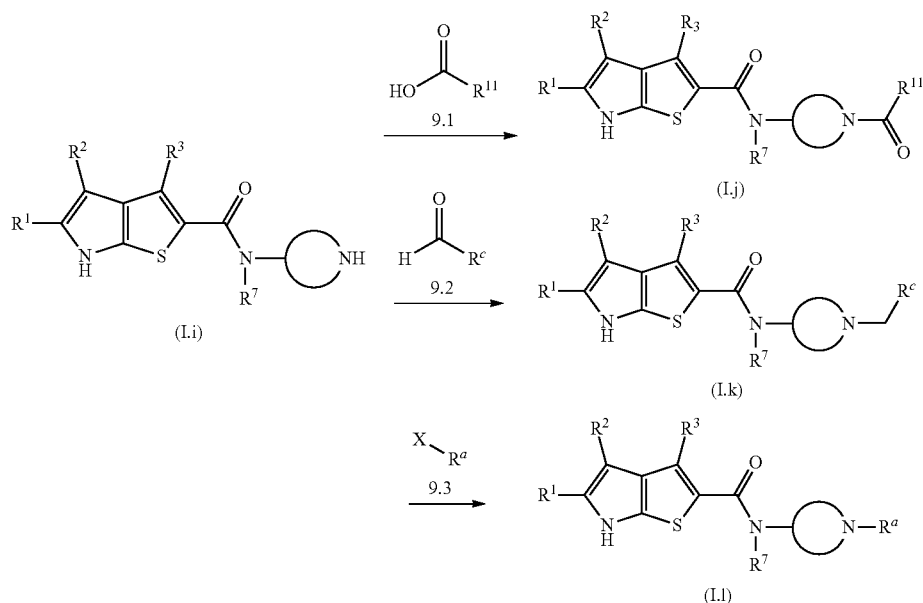
General Reaction Scheme 9
