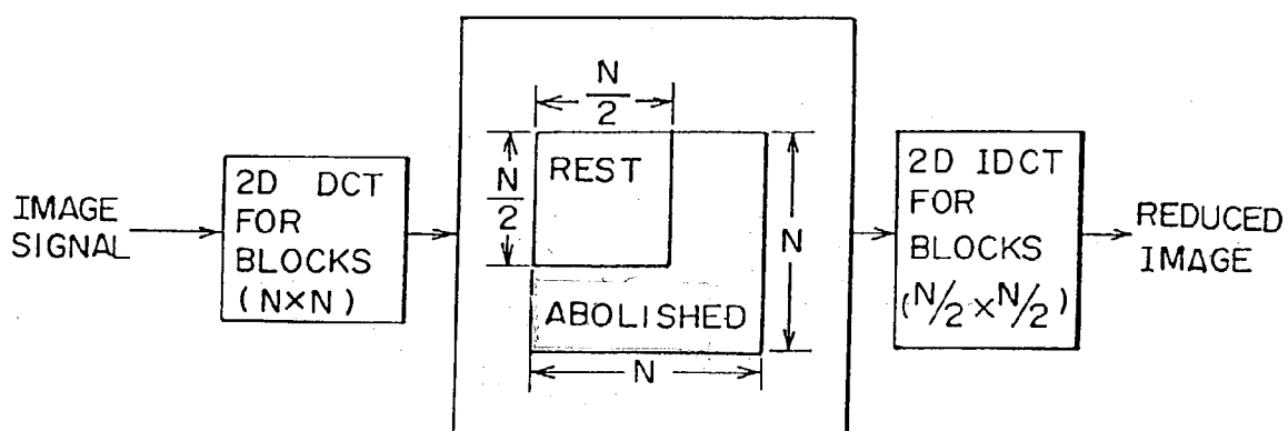
FIG. 59 PRIOR ART
