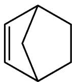
norbornene
