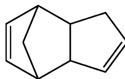
dicyclopentadiene
