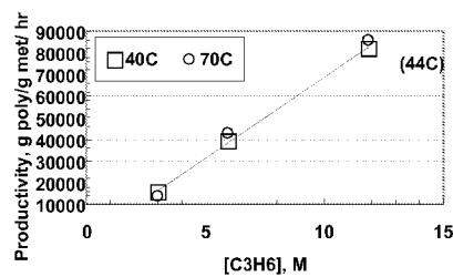
Figure 1 Productivity vs. propylene concentration
