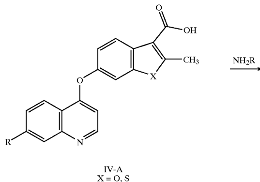
SCHEME IV: GENERAL PREPARATION OF CARBOXAMIDE ANALOGS (IV-B)
