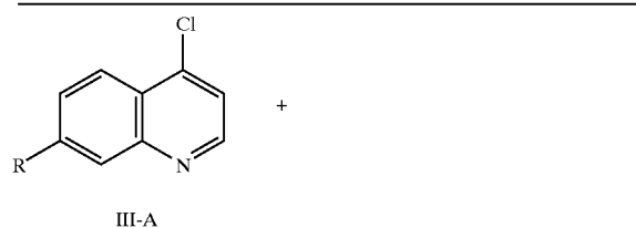
SCHEME III: GENERAL PREPARATION OF (INDOL-5-YL)QUINOLIN-4-AMINE (III-C)
