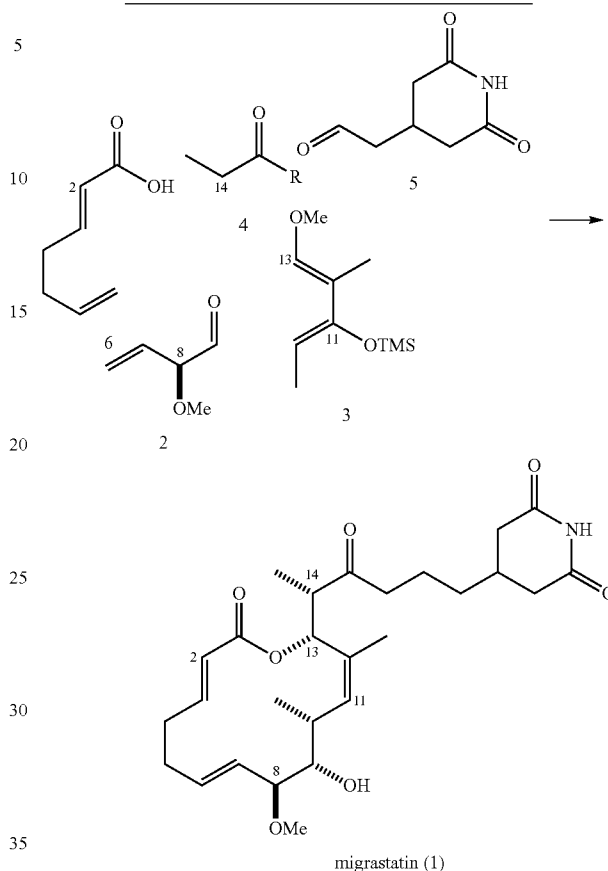
Scheme 17. Exemplary Strategy for the Assembly of Migrastatin
