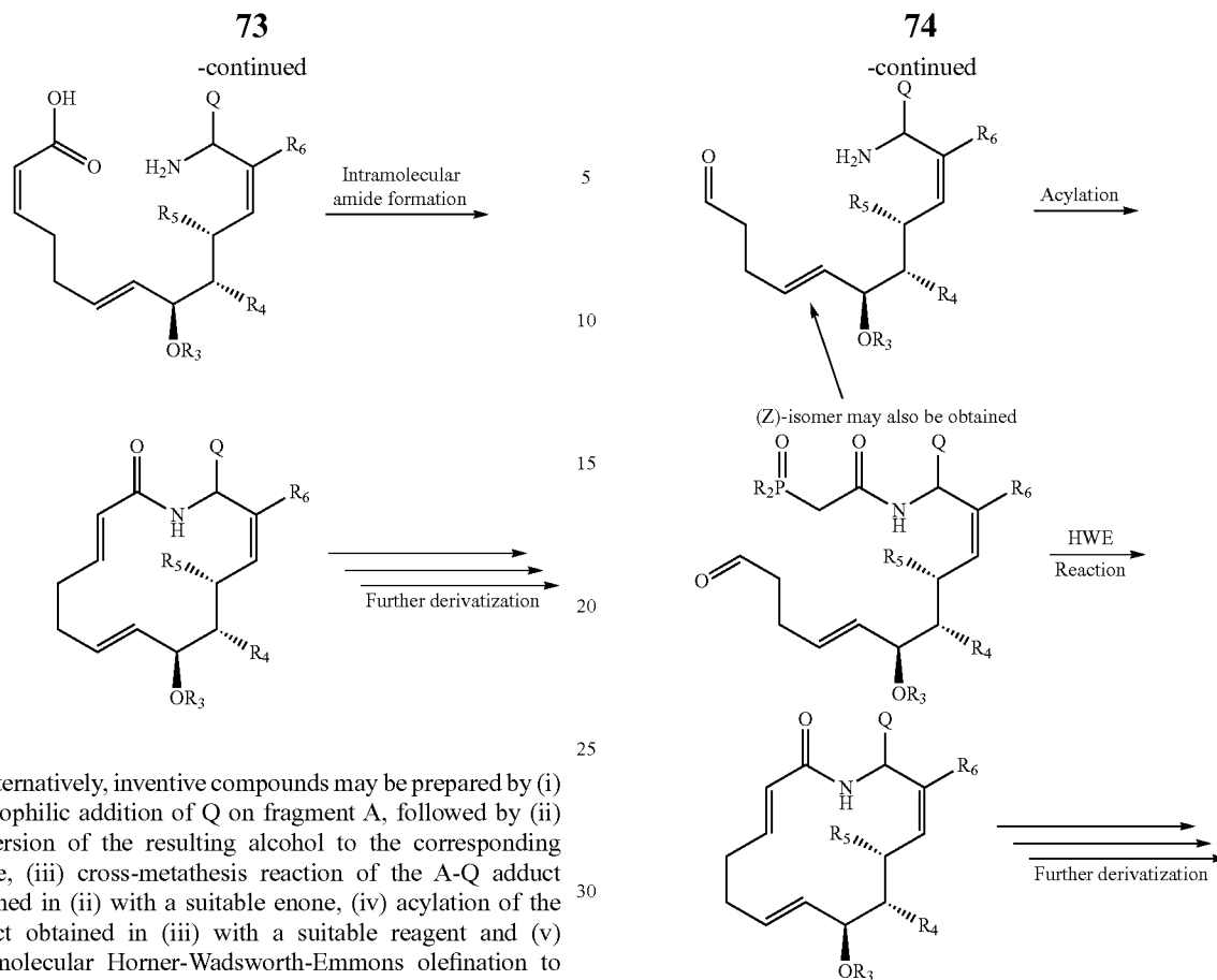
Scheme 15
