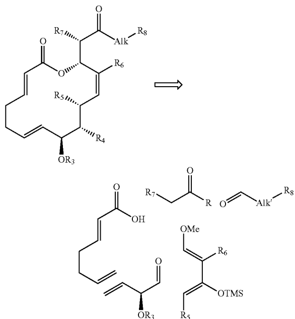
Scheme 1B
