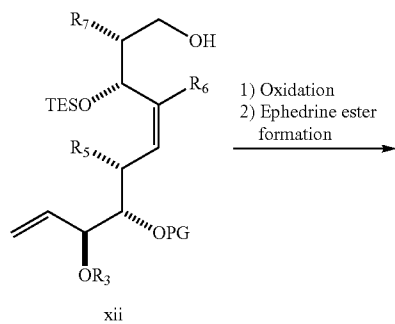
Scheme 9
