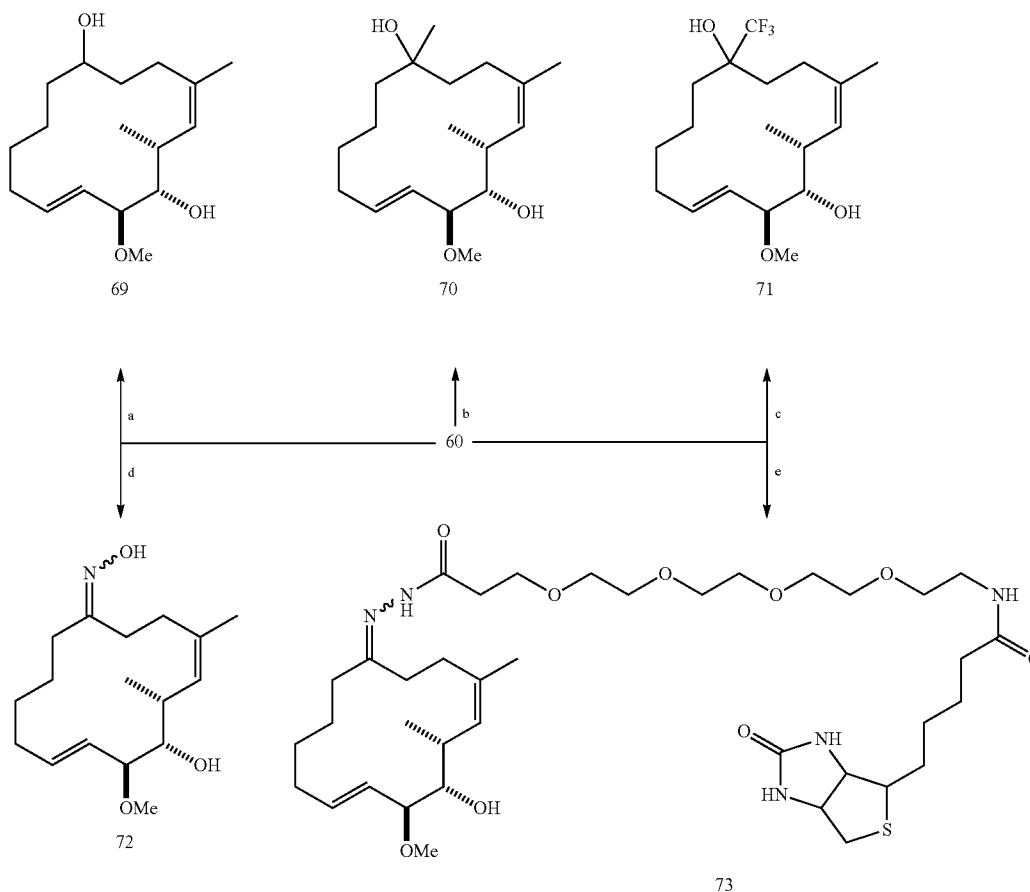
Scheme 30. Derivatization of Macroketone 60 a
