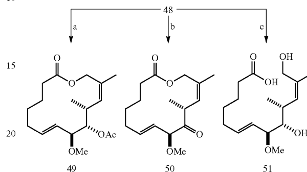
Scheme 27. Modification of Macrolactone 48 at the C9 position and Hydrolysis of 48 a
