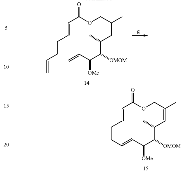
Scheme 18. A Model Study: Synthesis of the Migrastatin Core 15a
