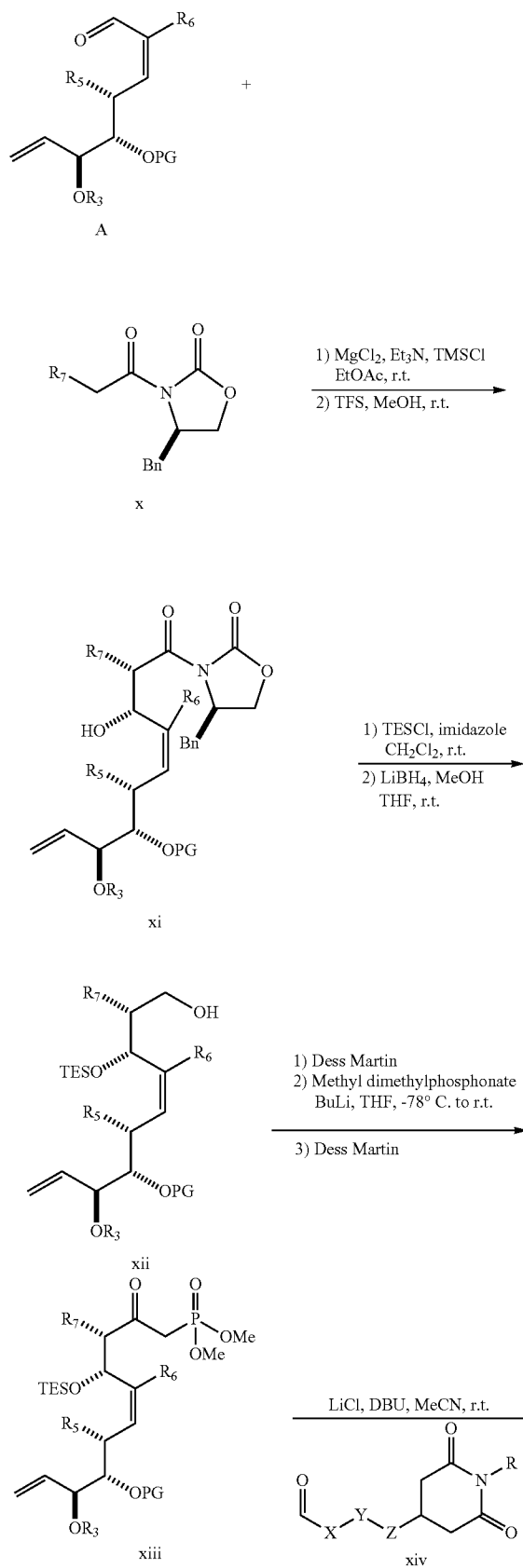
Scheme 5
