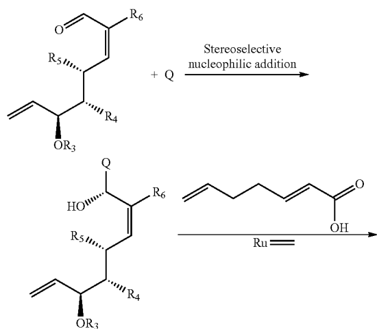
Scheme 11
