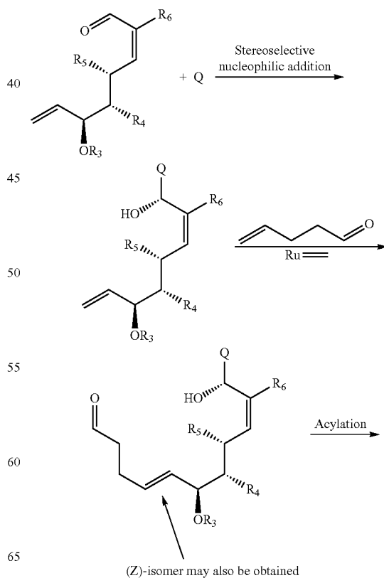
Scheme 12
