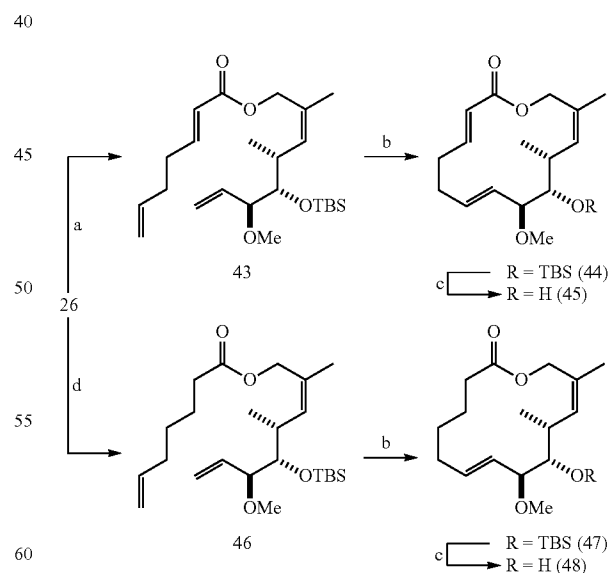
Scheme 25. Synthesis of Migrastatin Core 45 and Macrolactone 48 a
