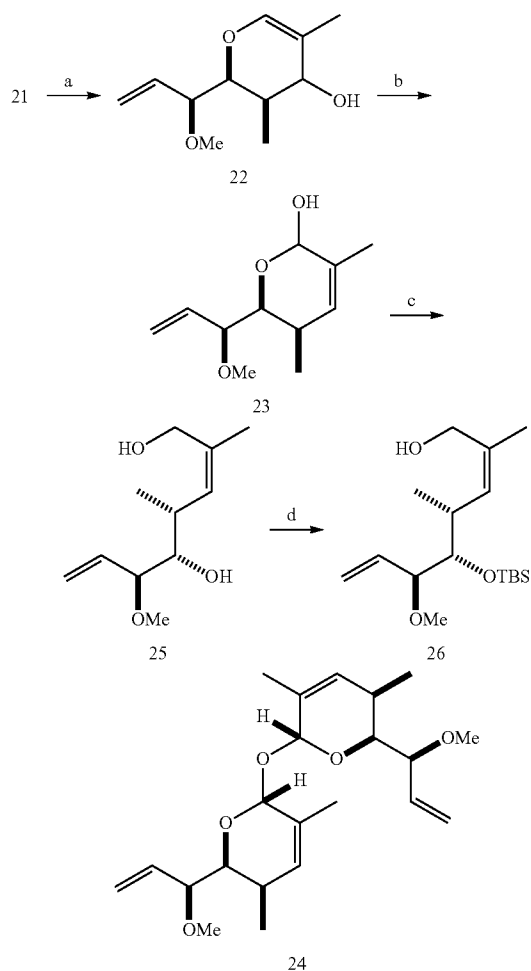
Scheme 20. Synthesis of Intermediate 26 a
