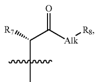
Scheme 1B
