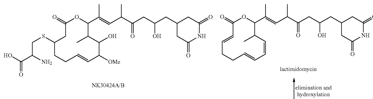
Scheme 16. Structure of Migrastatin and Related Natural Products
