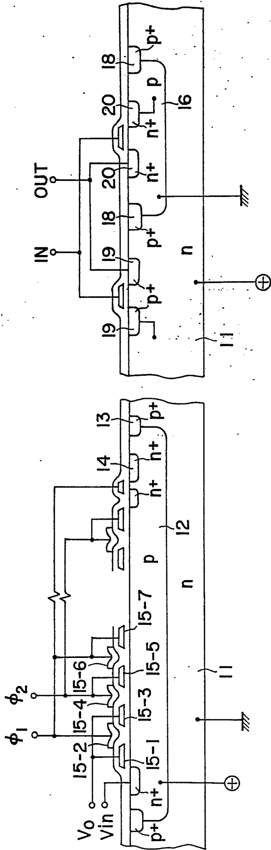
FIG. 1 PRIOR ART
