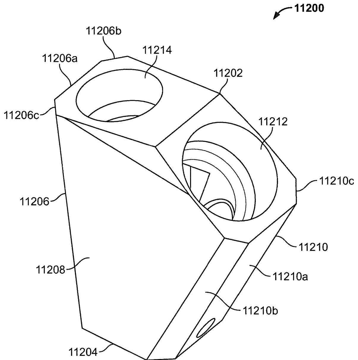
FIG. 112 (Prior Art)
