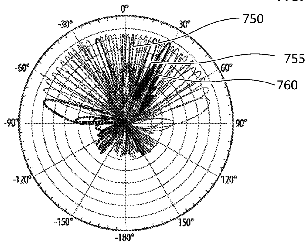
TYPICAL 40-BEAMS ORTHOGONAL-BEAM-SPACE CHANNELS
