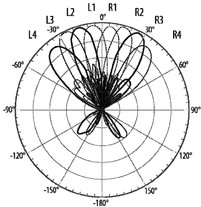
TYPICAL 8-BEAMS ORTHOGONAL-BEAM-SPACE CHANNELS
