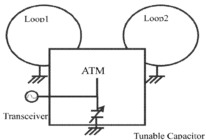
Two loop antenna configuration utilizing a single tunable capacitor and coupled to a common transceiver port
