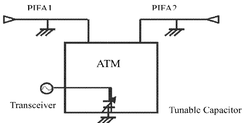
Two antenna configuration utilizing a single tunable capacitor and coupled to a common transceiver port
