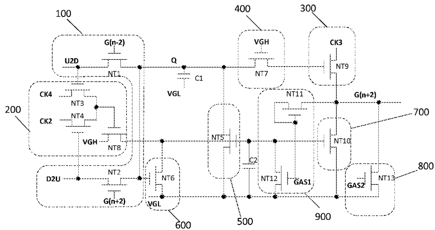
FIG. 3 (PRIOR ART)
