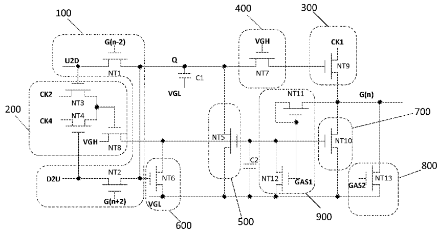
FIG. 2 (PRIOR ART)
