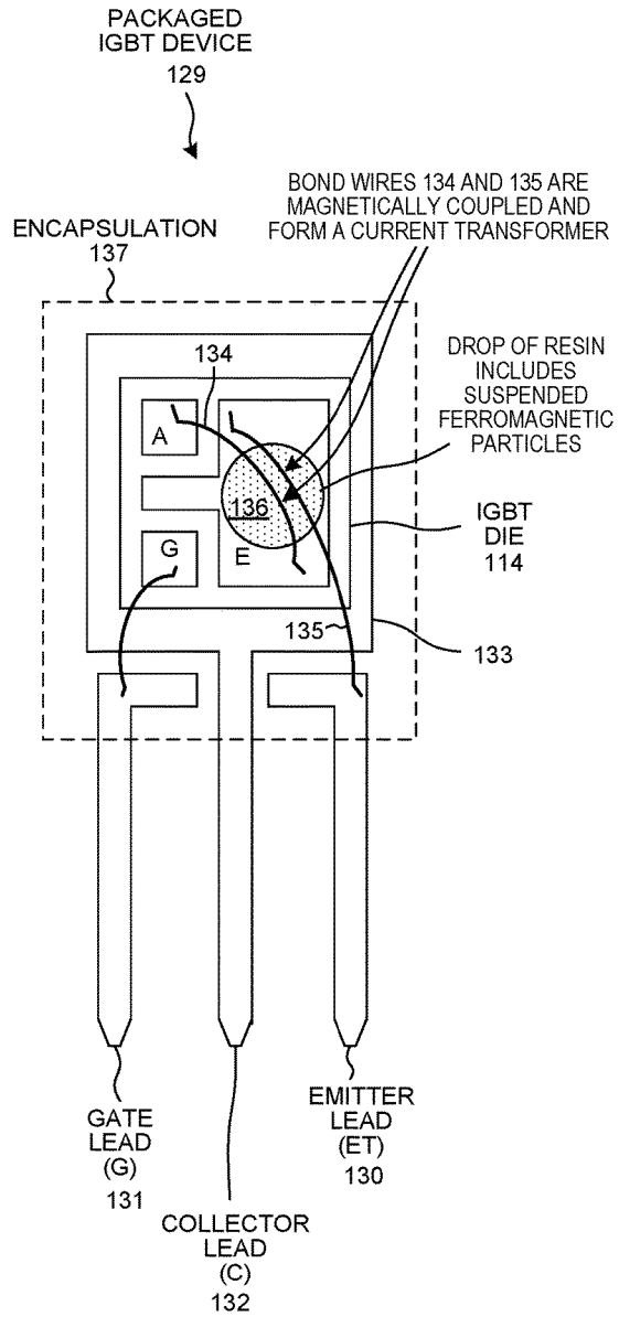
THREE-TERMINAL PACKAGED IGBT HAVING A CURRENT TRANSFORMER
