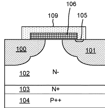
CROSS-SECTIONAL SIDE VIEW ALONG LINE A-A OF FIG. 11A
