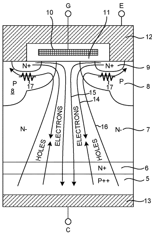
IGBT (PRIOR ART)
