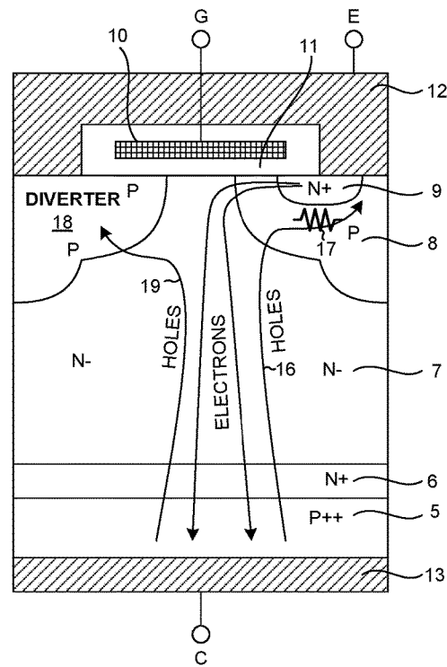
IGBT WITH HOLE DIVERTER (PRIOR ART)
