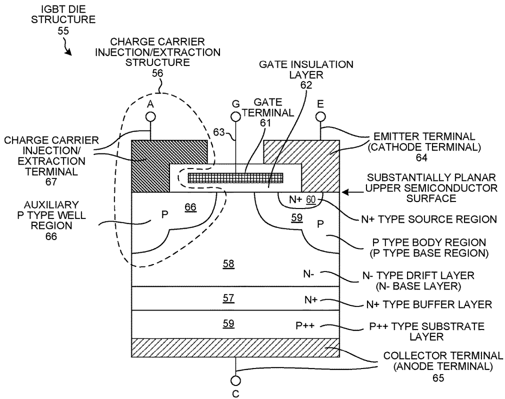
IGBT WITH CHARGE CARRIER INJECTION/EXTRACTION STRUCTURE
