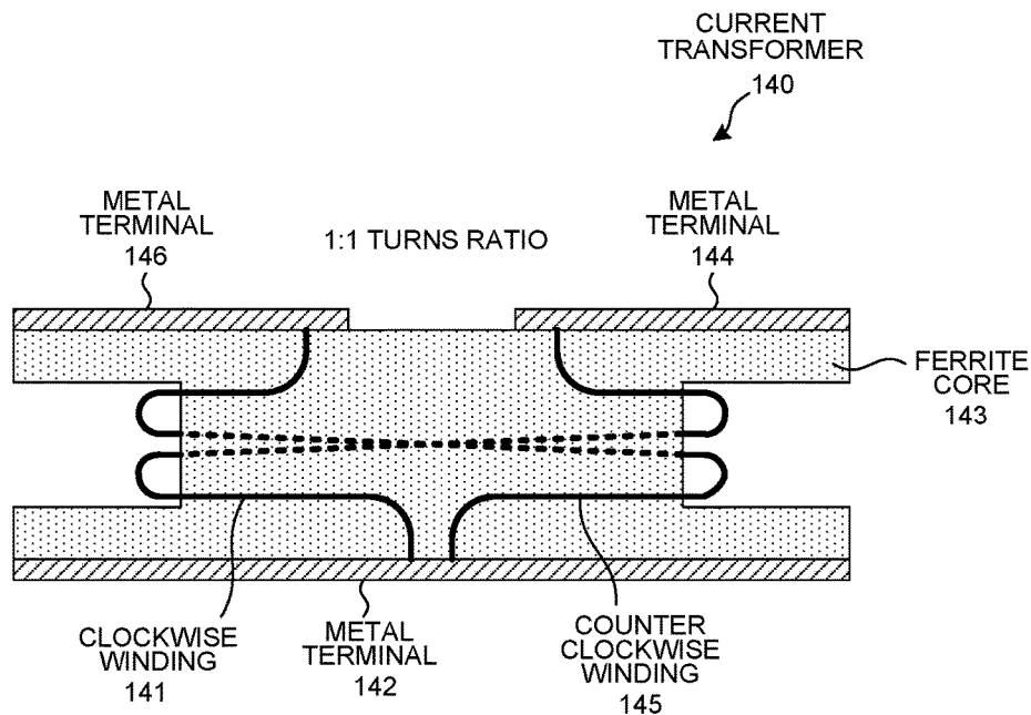
CROSS-SECTIONAL DIAGRAM OF CURRENT TRANSFORMER
