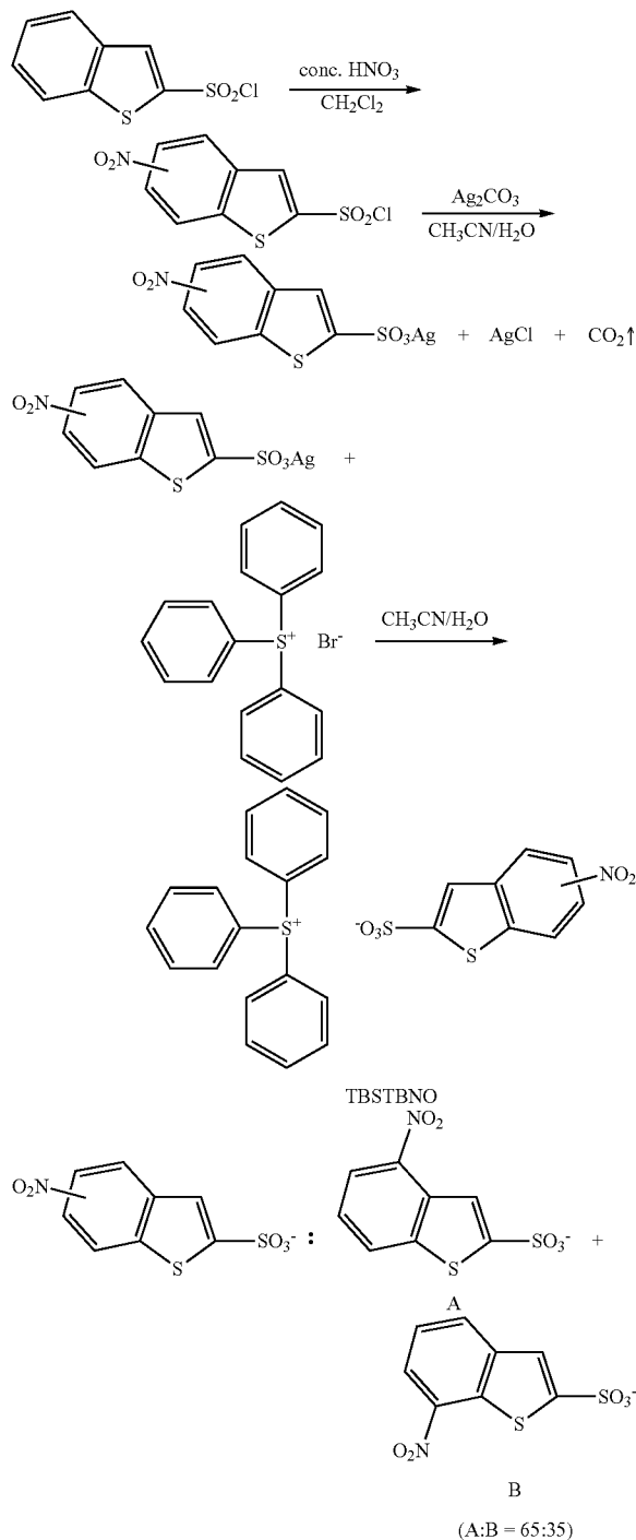
Scheme 1. Synthesis of fluorine-free fused-ring heteroaromatic PAGs.
