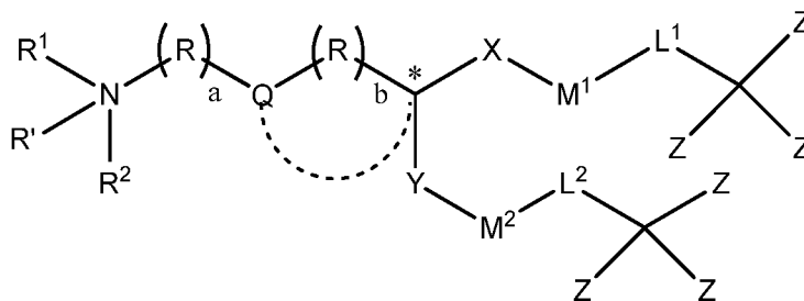
Formula (IV)
