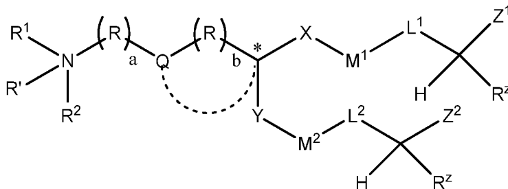
Formula (IIIA)
