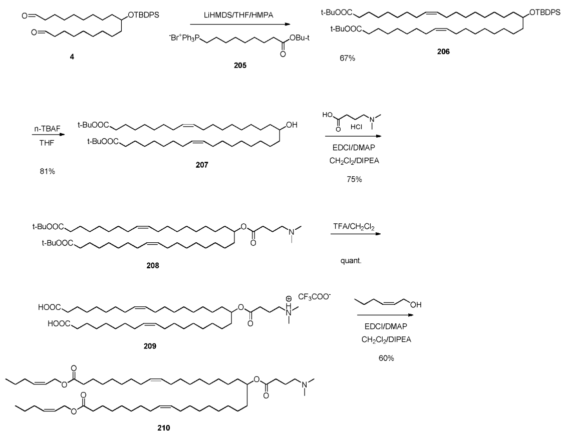
Scheme 10
