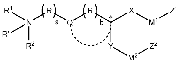
Formula (VII)
