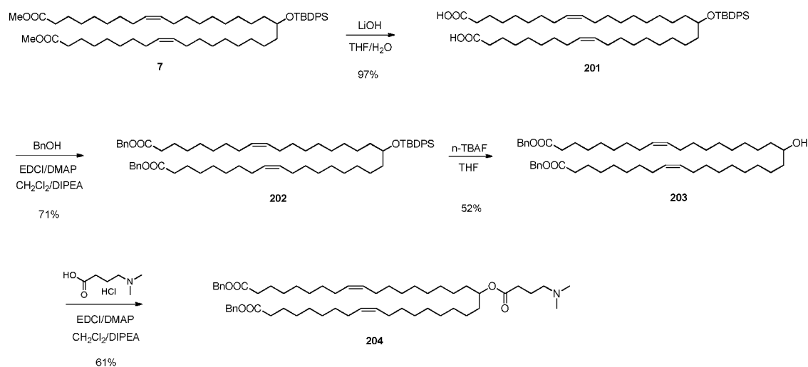
Scheme 9
