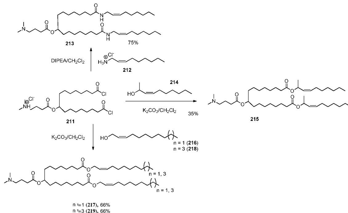
Scheme 11
