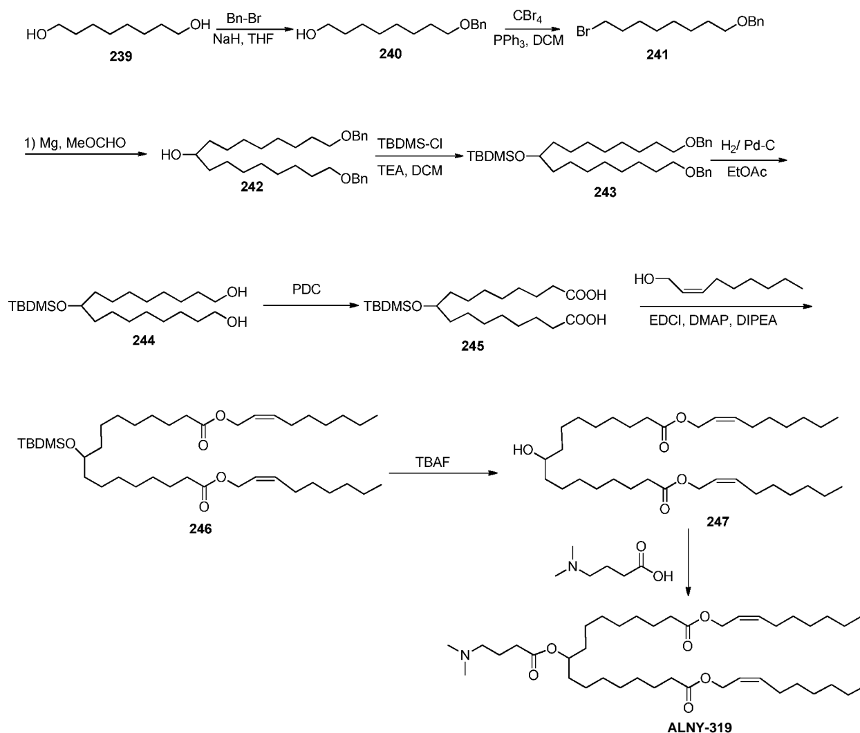
Scheme 17:
