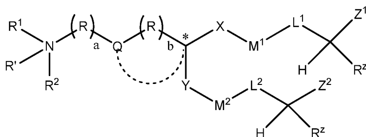
Formula (III)
