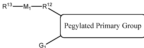
Formula (IX)
