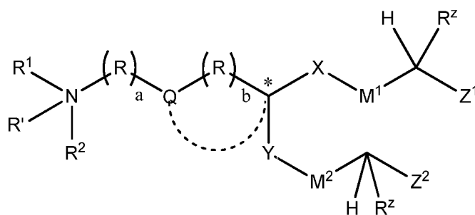
Formula (II)
