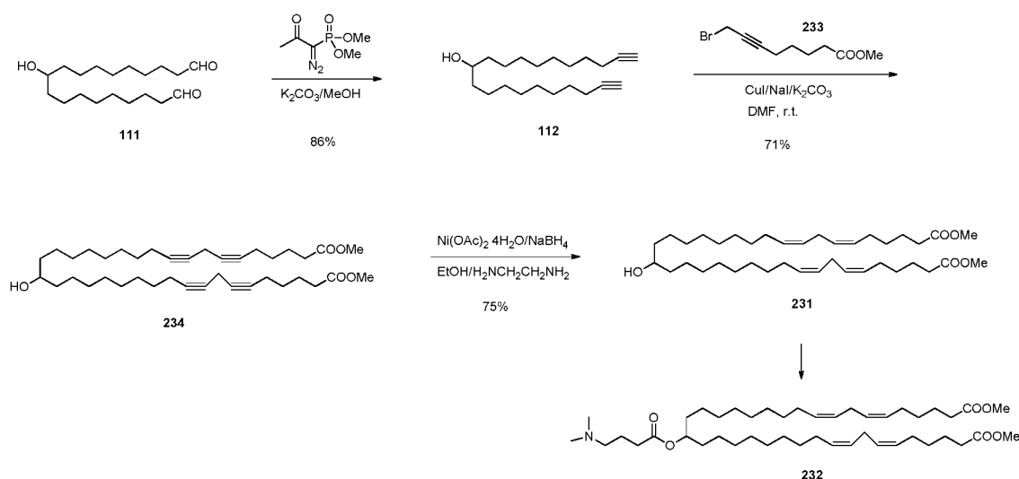
Scheme 15
