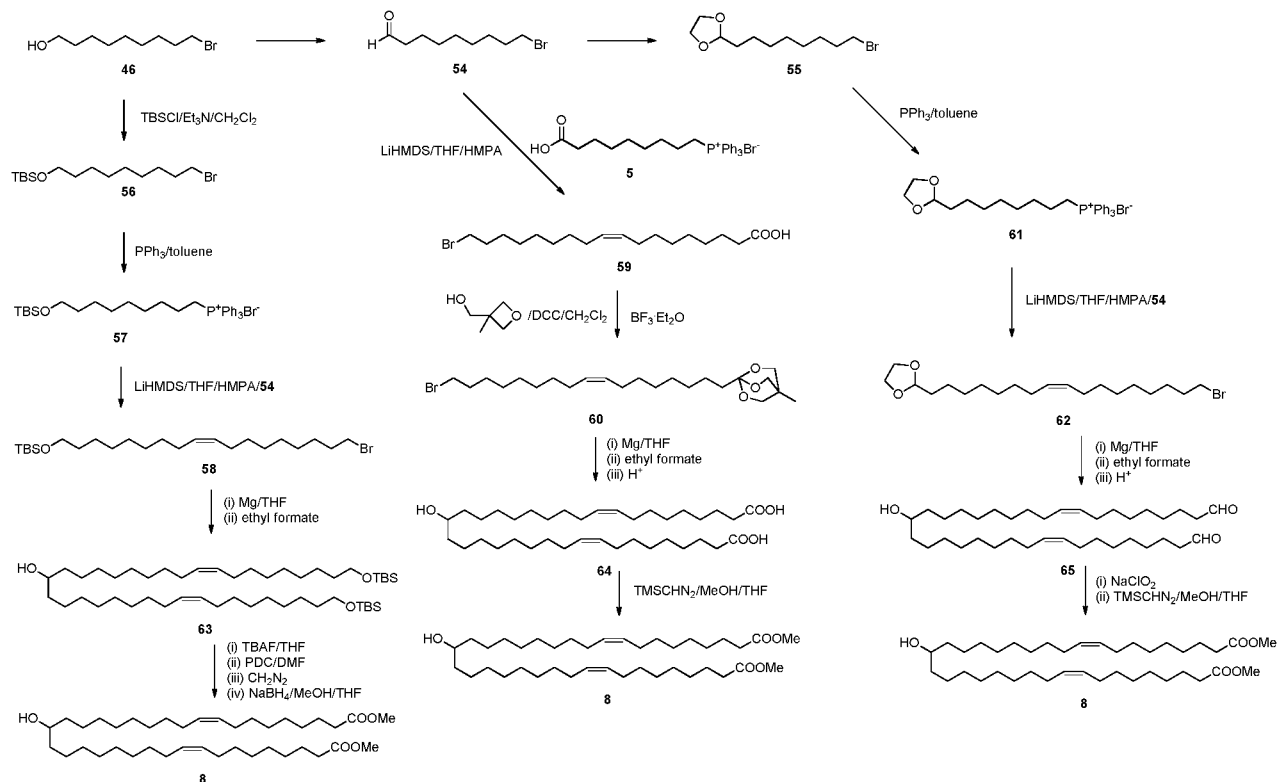
Scheme 6
