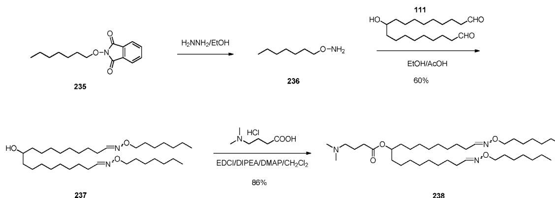
Scheme 16
