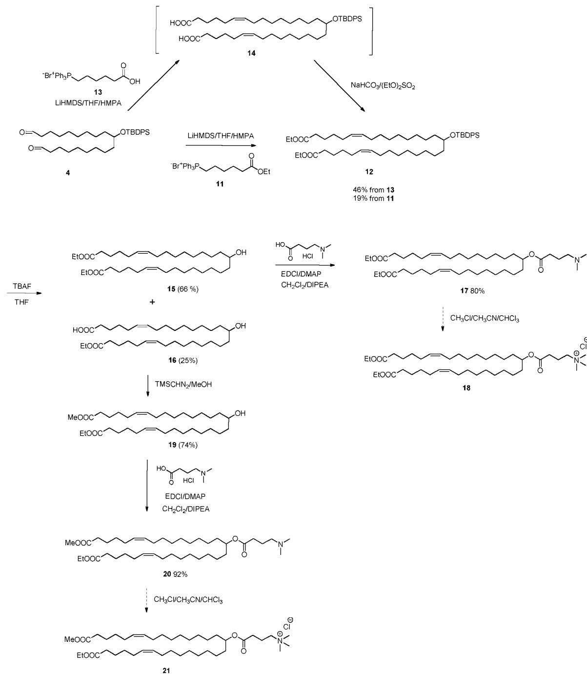
Scheme 2
