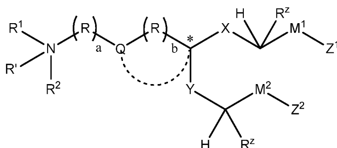
Formula (I)
