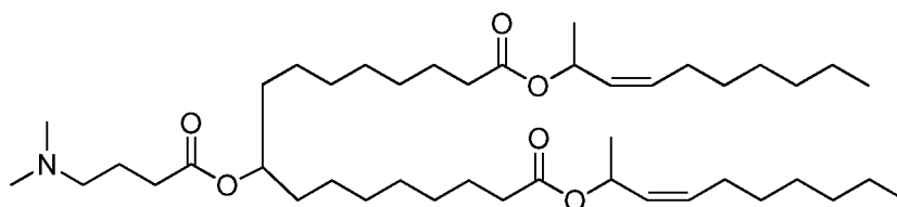
(Compound 1)
