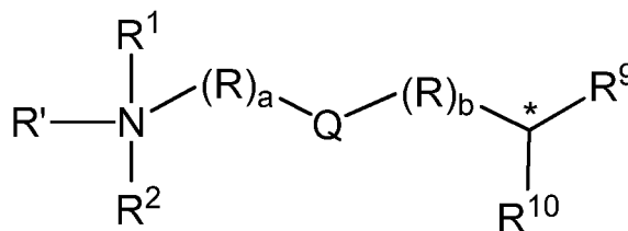
Formula (VIA)
