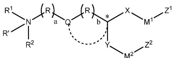
Formula (V)
