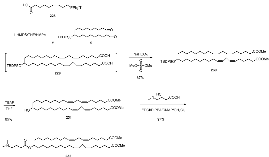
Scheme 14
