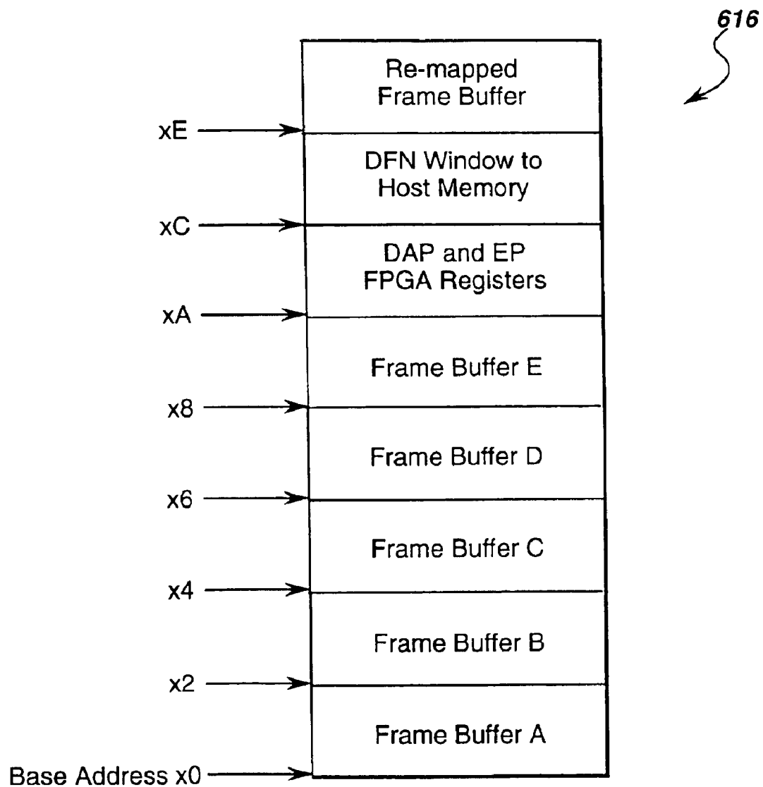
Mapping of 16 MByte PCI Address Space
