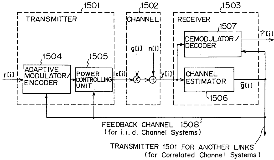
SYSTEM MODEL FIG. 1A
