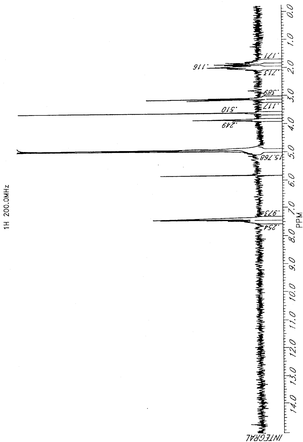
1 H nuclear magnetic resonance spectrum obtained from Form I
