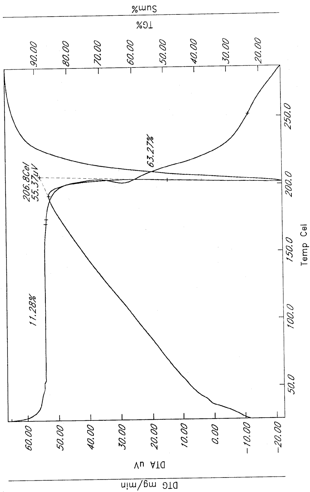
FIG. 3 Thermogravimetric Gravimetric/Differential Thermal Analysis of Form I
