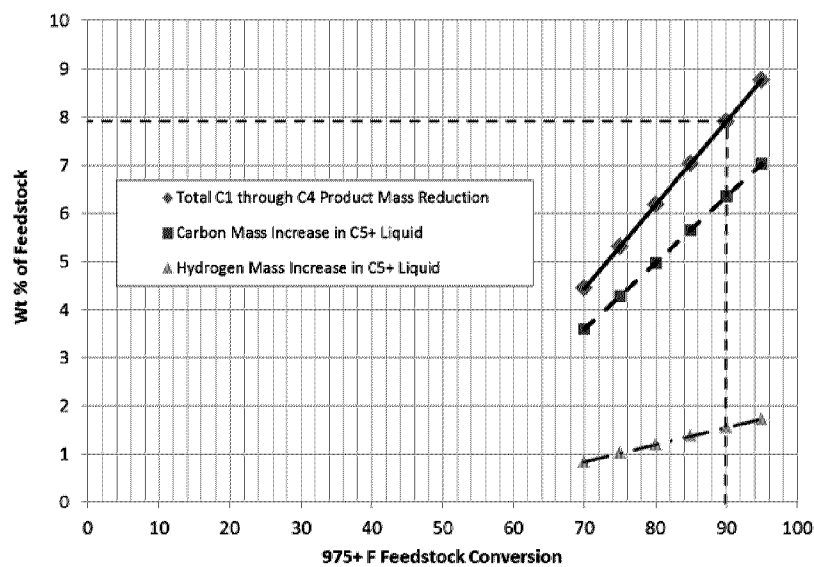
C1-C4 Mass Transferred to C5+ Liquid Yield (Relative to Base Commercial Operation)
