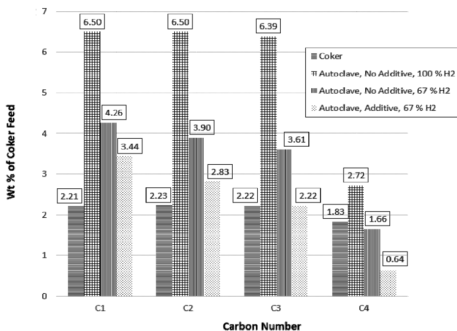
Thermal C1 – C4 Yields
