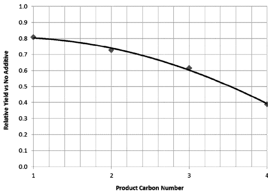
Reduction Of C1 to C4 Carbon Yield With Additive Addition (67 % hydrogen partial pressure reference)
