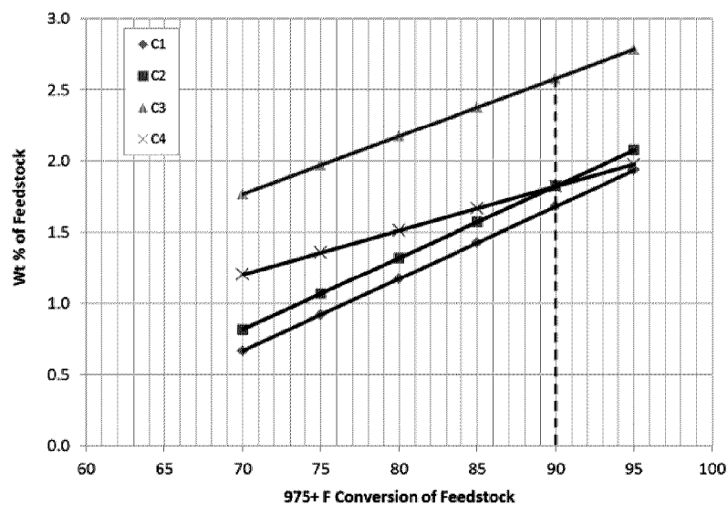
FIG. 22A Mass Transferred to C5+ Liquid Yield by Carbon Number
