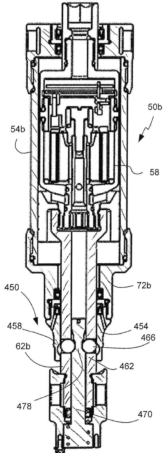
Fig. 17d unlocked
