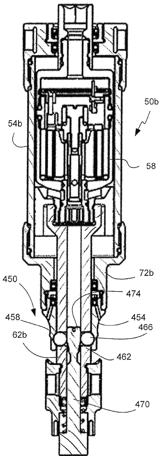
Fig. 17c locked
