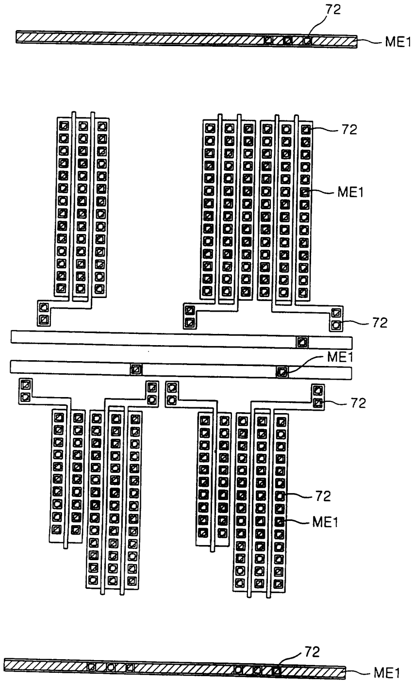
FIG. 8(PRIOR ART)
