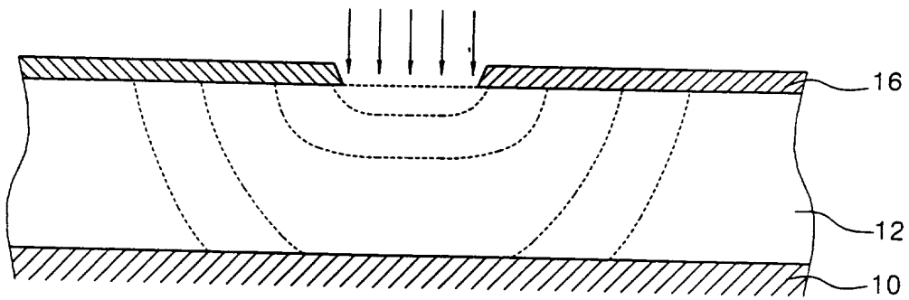
FIG. 2 (PRIOR ART)
