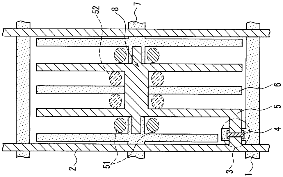
FIG. 5A (Feeding Side)
