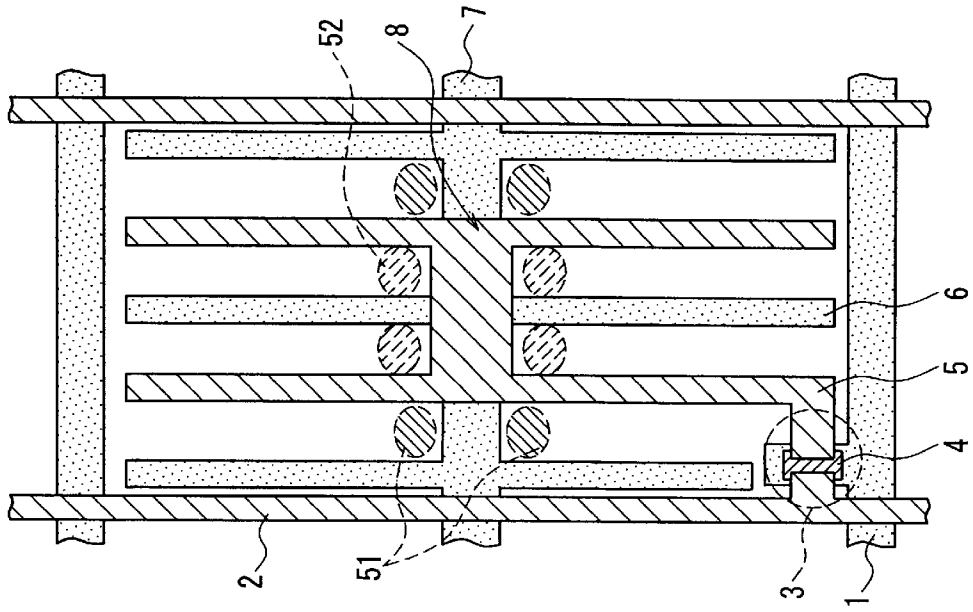
FIG. 5B (Termination Side)
