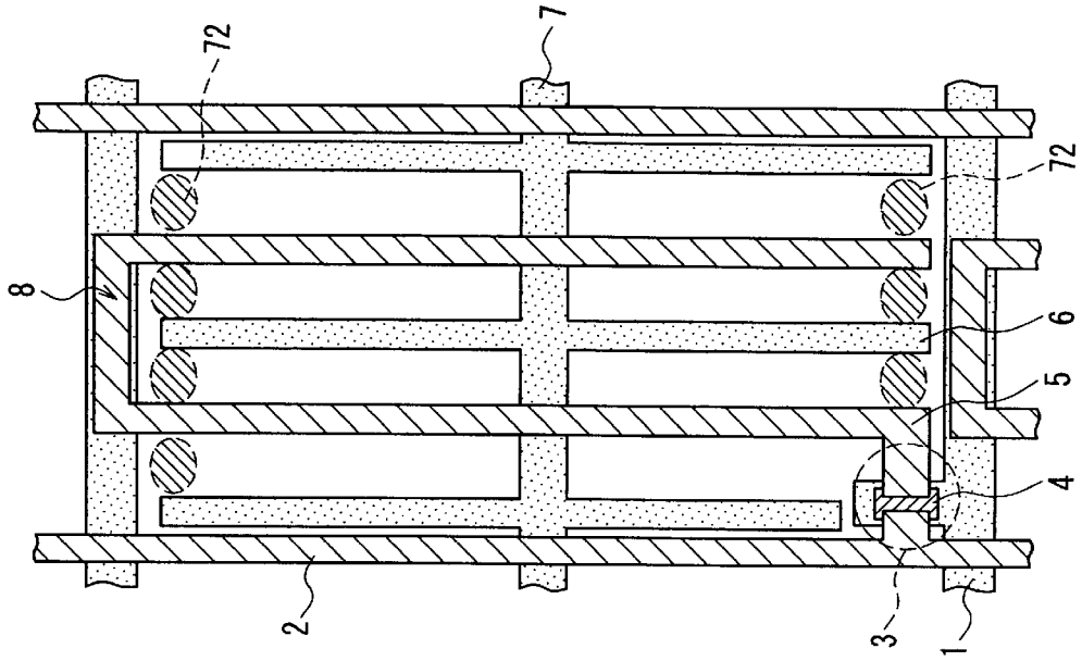
FIG. 7B (Termination Side)
