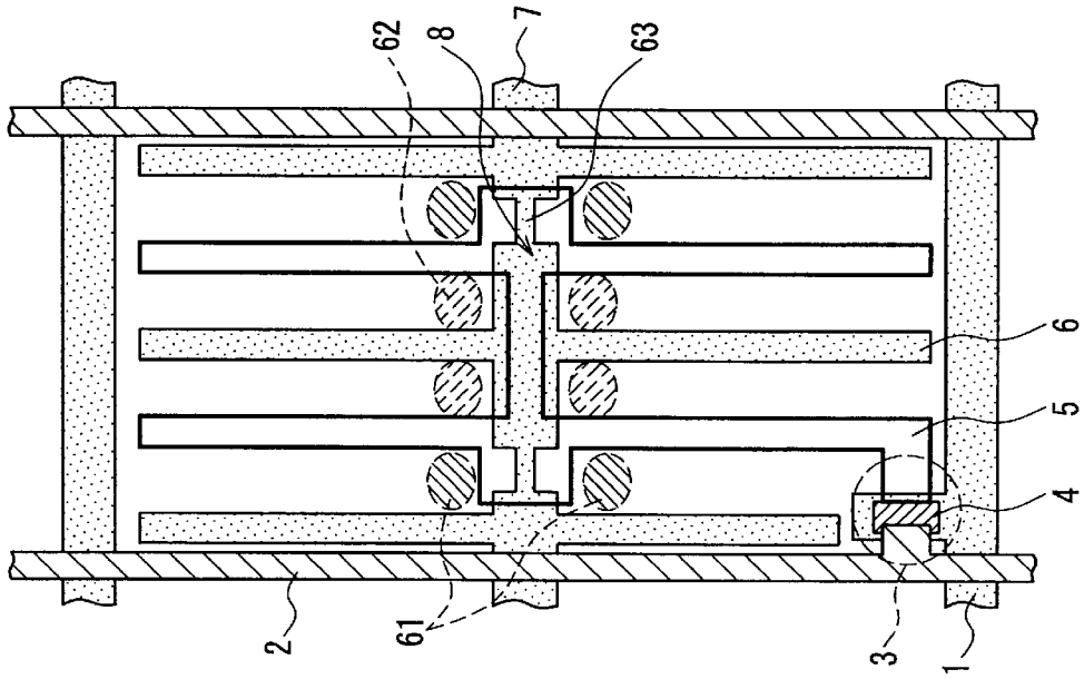
FIG. 6B (Termination Side)
