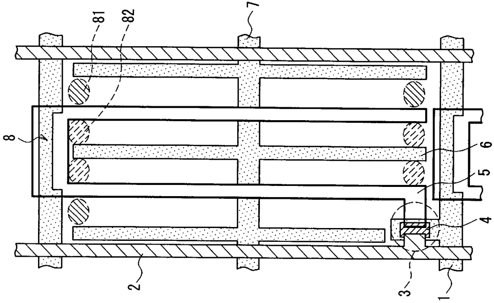
FIG. 8B (Termination Side)
