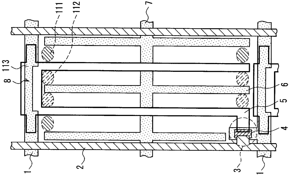
FIG. 11B (Termination Side)
