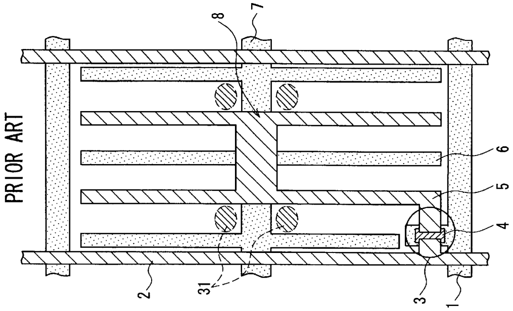
FIG. 3B (Termination Side)
