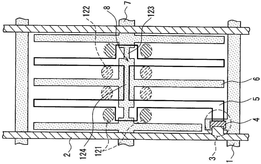
FIG. 12B (Termination Side)
