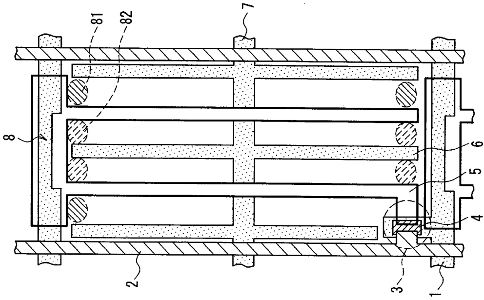
FIG. 9B (Termination Side)
