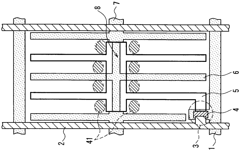
FIG. 4B (Termination Side)
