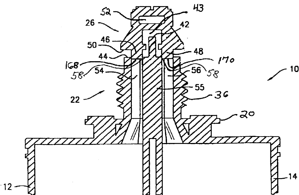
FIG. 4 (PRIOR ART)
