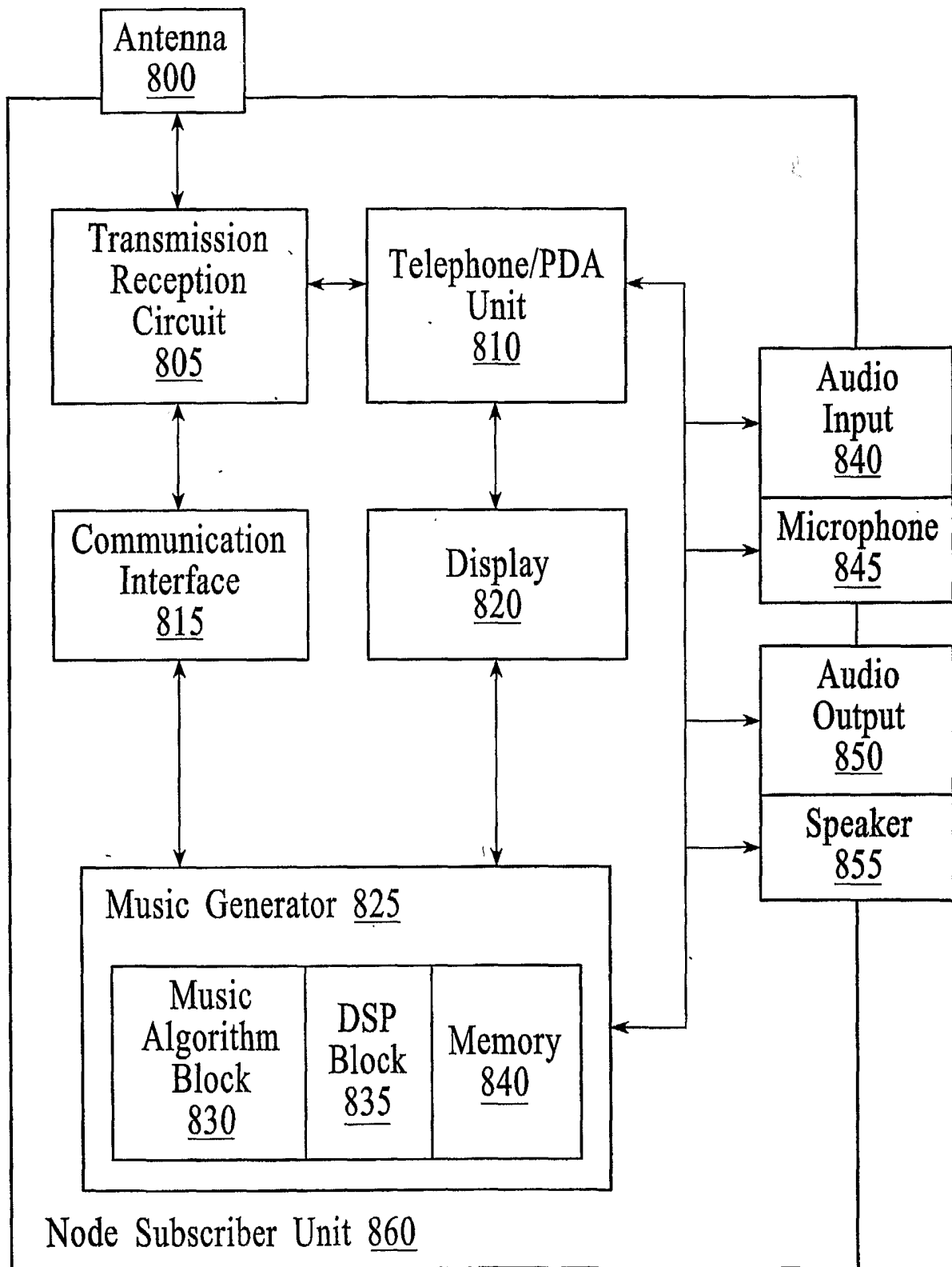
Node/Subscriber Unit Functional Blocks
