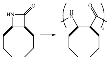
Reaction Scheme 3
