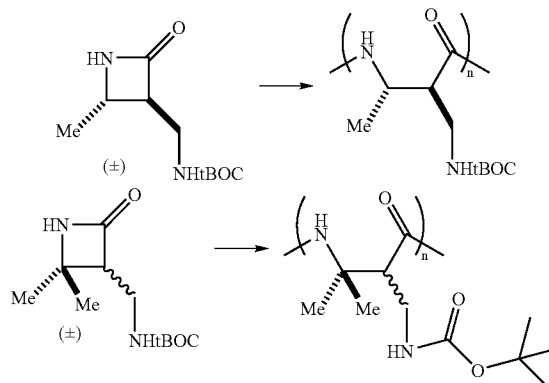
Reaction Scheme 5
