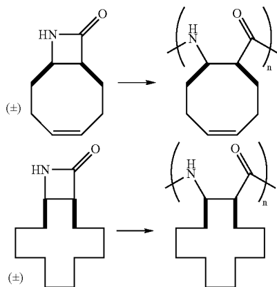
Reaction Scheme 4
