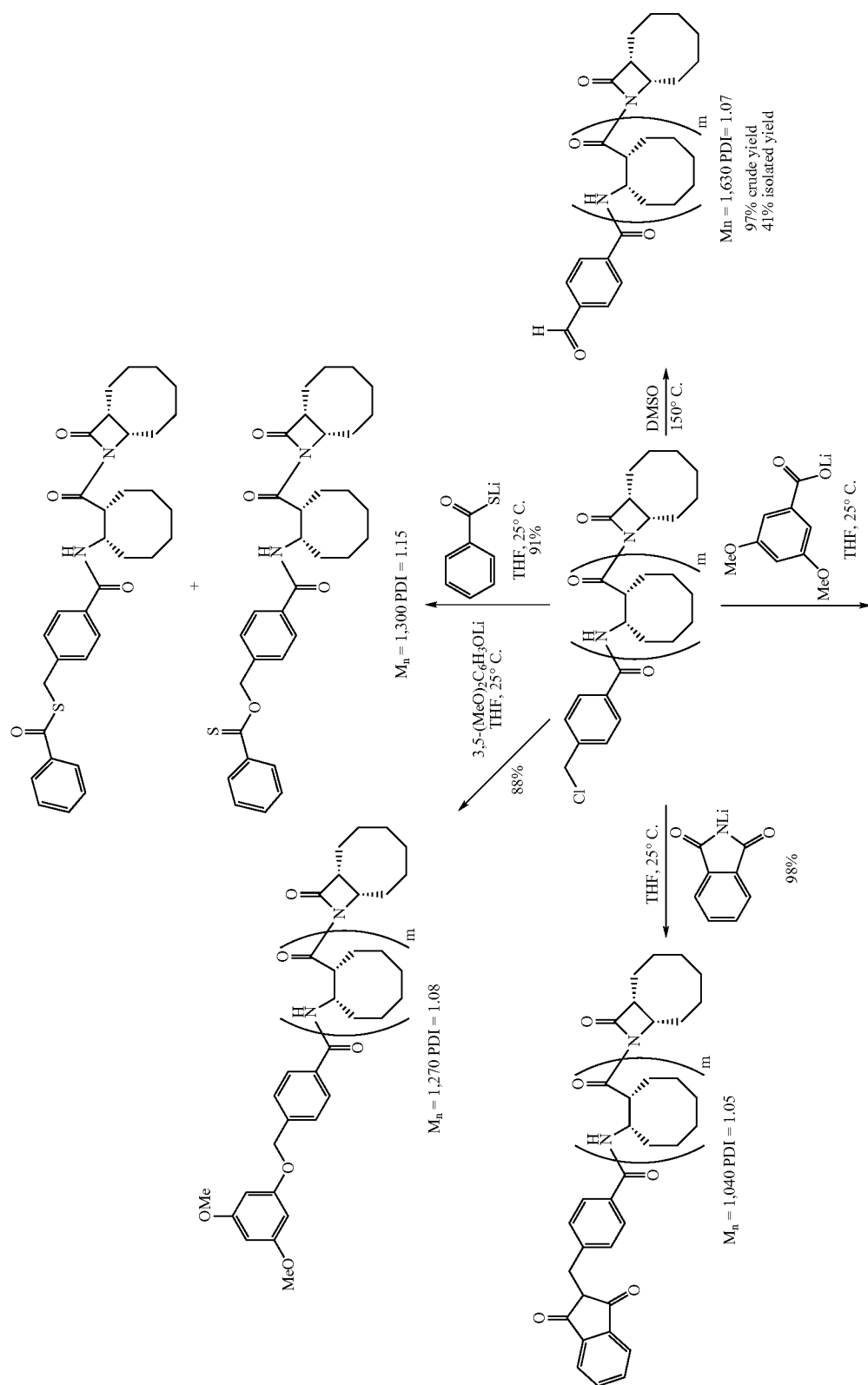
Reaction Scheme 8
