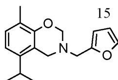
Bz-FA-carvacrol (3)
