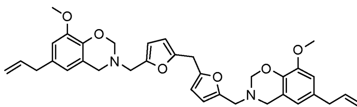
Bz-DFDA-eugenol (5)
