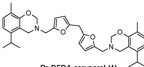
Bz-DFDA-carvacrol (4)
