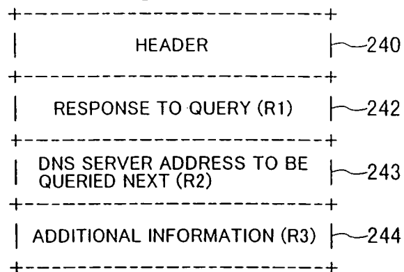
DNS response message format
