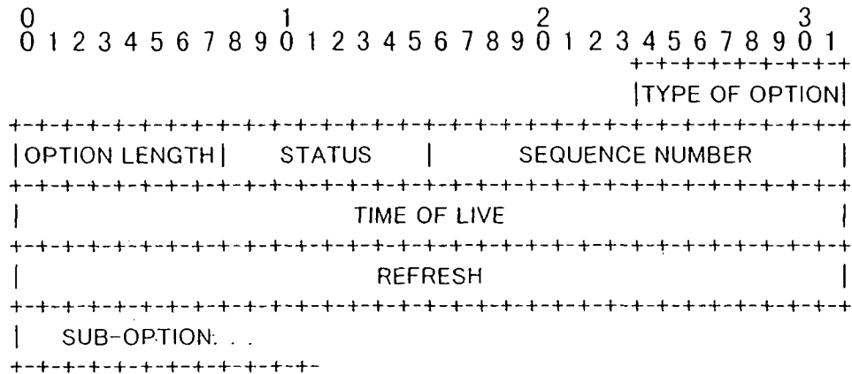
Mobile IPv6 binding acknowledge message format
