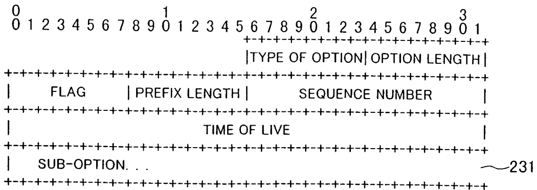
Mobile IPv6 binding update message format
