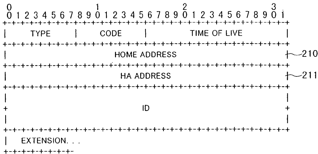
mobile IPv4 registration reply message format
