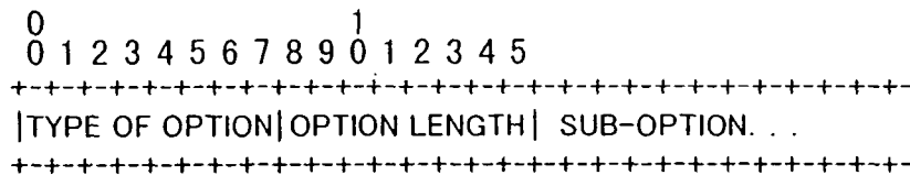
Mobile IPv6 binding request message format
