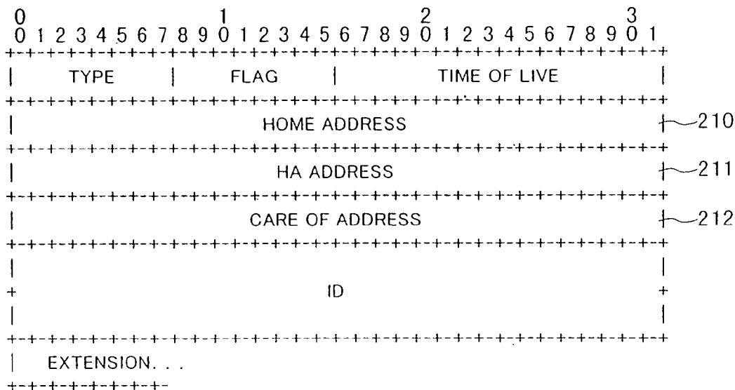
mobile IPv4 registration request message format
