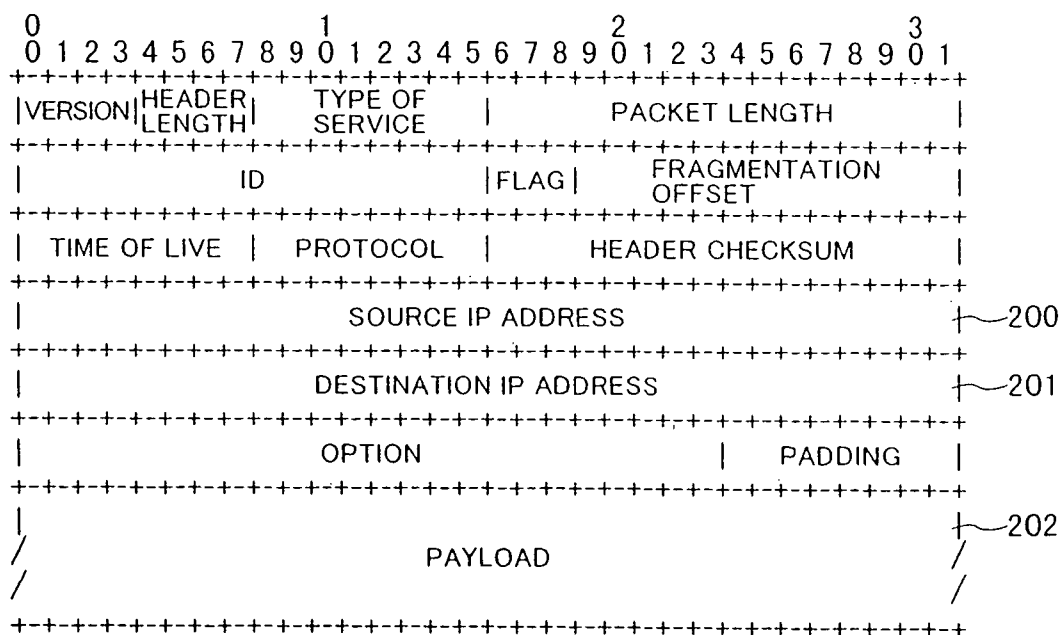
IPv4 packet format
