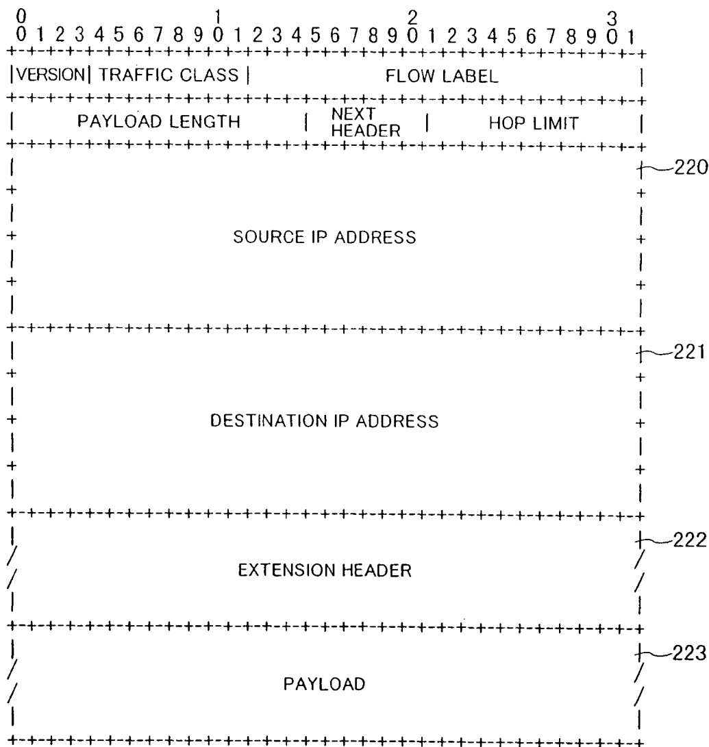
IPv6 packet format
