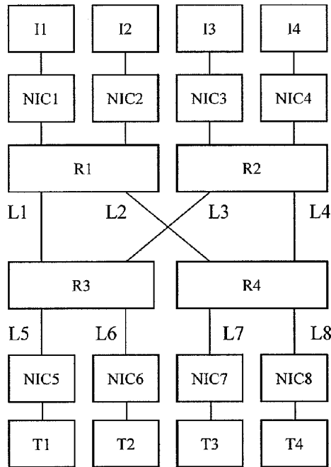
FIG. 1 (conventional art)
