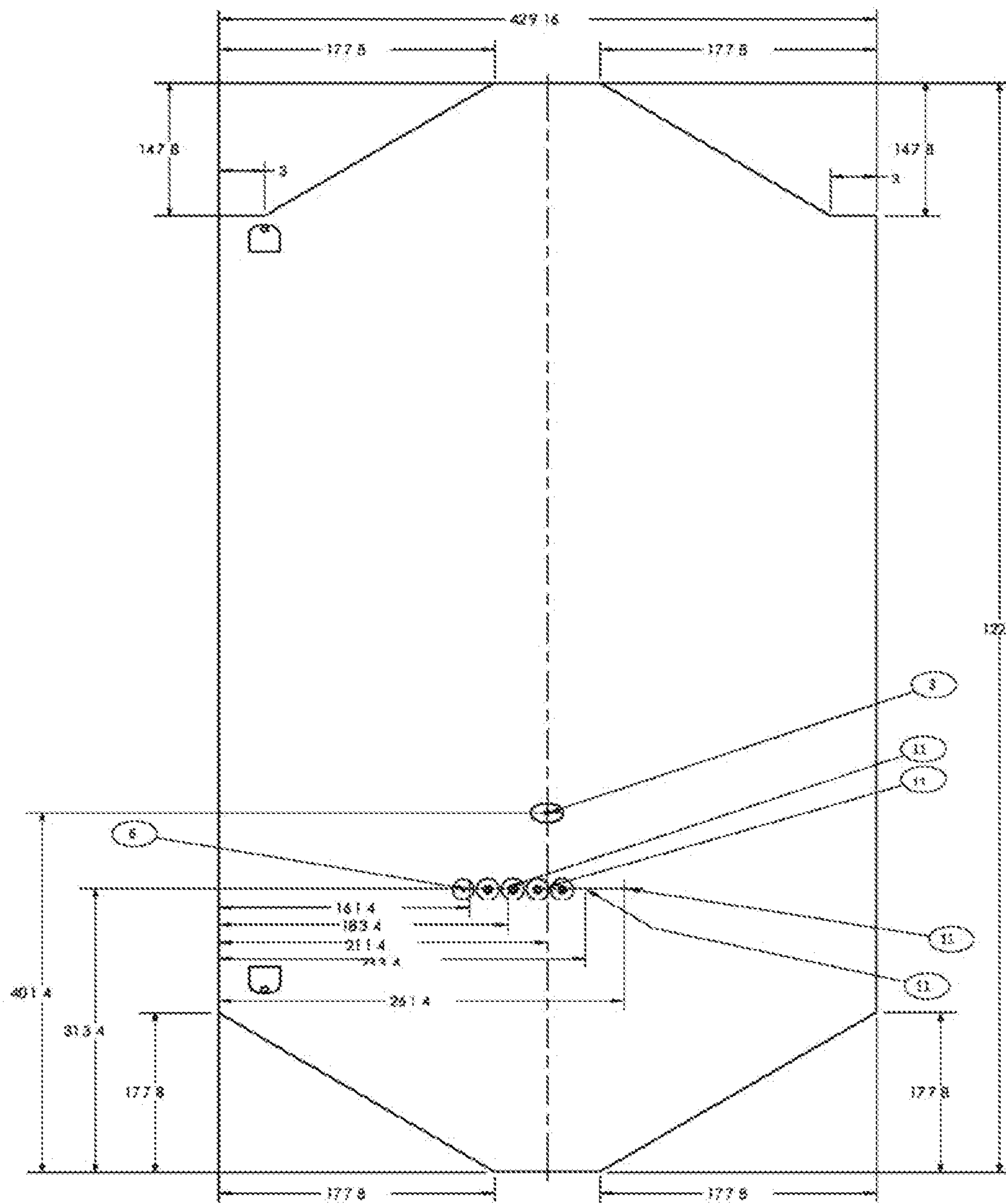
Front Panel (Trapezoidal) Exterior View
