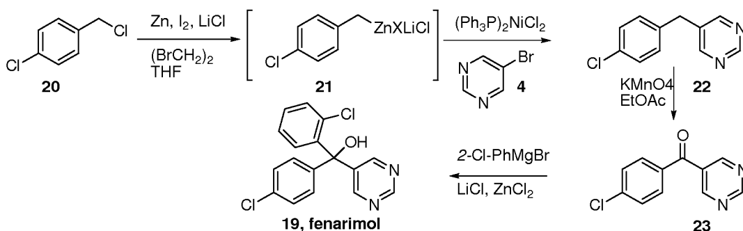
Scheme 5. Synthesis of fenarimol ( 19 )
