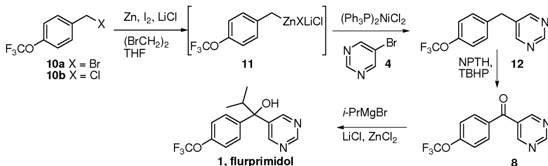
Scheme 3. Synthesis of flurprimidol ( 12 ).
