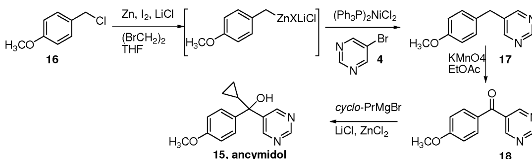
Scheme 4. Synthesis of ancymidol ( 15 ).
