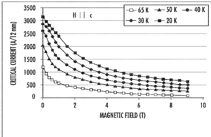
FIELD DEPENDENCE OF I_c AT 20 - 65K 2011 SUPERPOWER AP WIRE
