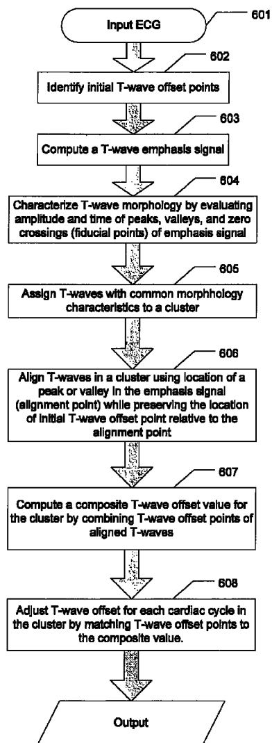
Figure 6 - Computing an adjusted T-wave offset
