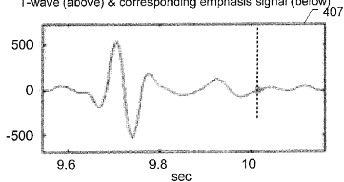
T-wave (above) & corresponding emphasis signal (below)
