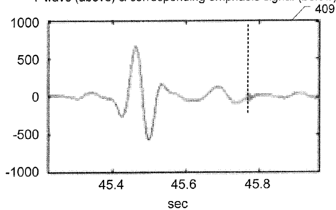
T-wave (above) & corresponding emphasis signal (below)
