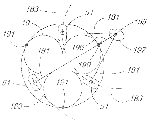
Trim Mode (Greater Than Zero Radius) FIG. 20
